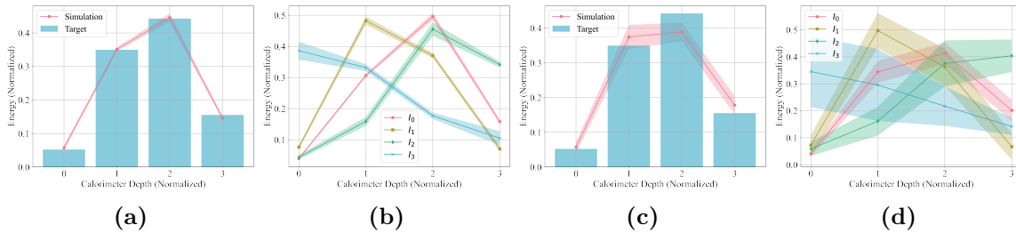
Figure 4: Mean (a,c) and individual images (b,d) obtained by inference test on ibmq_jakarta (a,b) and IONQ (c,d).
