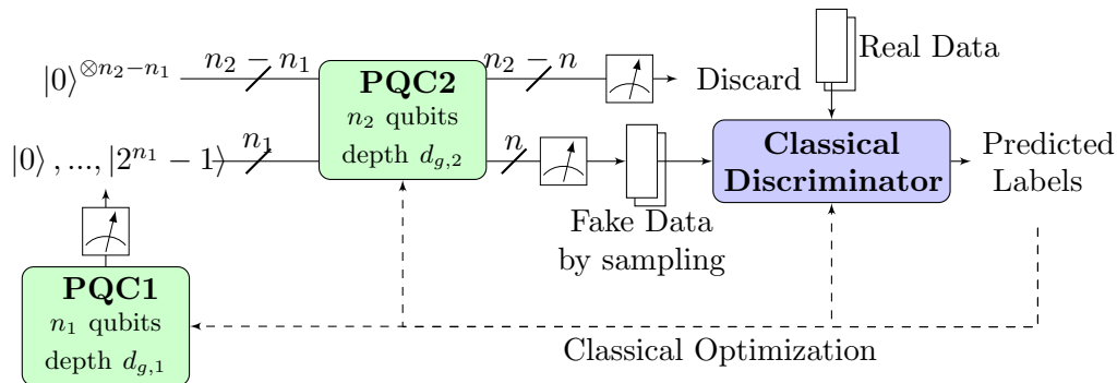
Figure 1: Schematic Diagram of dual-PQC GAN to reproduce images of 2^n pixels.
