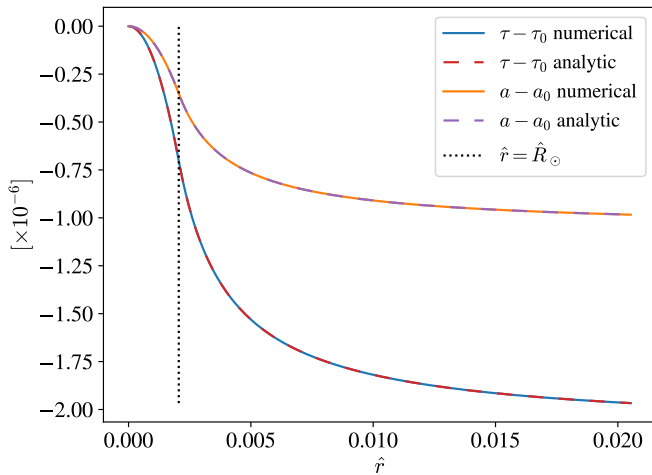
FIG. 1: The field profiles for \hat{R} = \hat{R}_\odot , \kappa = 1 and \epsilon = 0.5 . The initial values are taken such that \tau_0 = a_0 = 1 , \tau'(0) = a'(0) = 0 .
