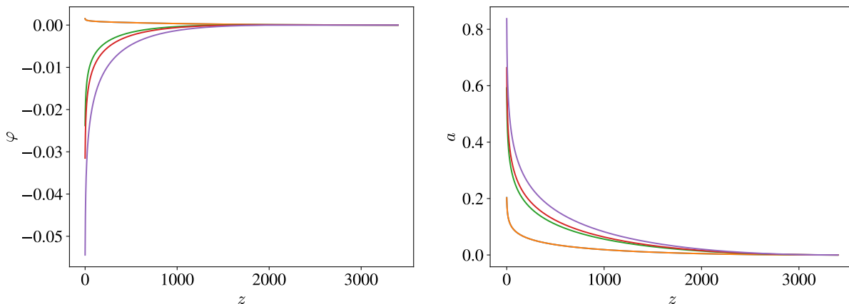
FIG. 4: The Field evolutions for \kappa = 10^{-3} and \epsilon_B = 10^{-3} as a function of the redshift z defined in the baryon frame. The values of \epsilon_C and \hat{\rho}_\Lambda for each colour are given in Fig.3.
