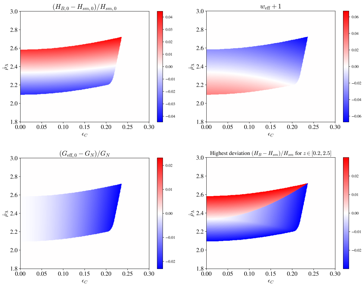
FIG. 2: We show the values of the parameters which satisfy the cosmological tests for \kappa = 10^{-3} and \epsilon_B = 10^{-3} . 602 \times 602 points are plotted. The coloured regions satisfy the four constraints: |\Delta H_0/H_0| < 0.1 , |\Delta w| < 0.1 , |\Delta G/G| < 0.4 , |\Delta H/H|_{\text{BAO}} < 0.03 .
