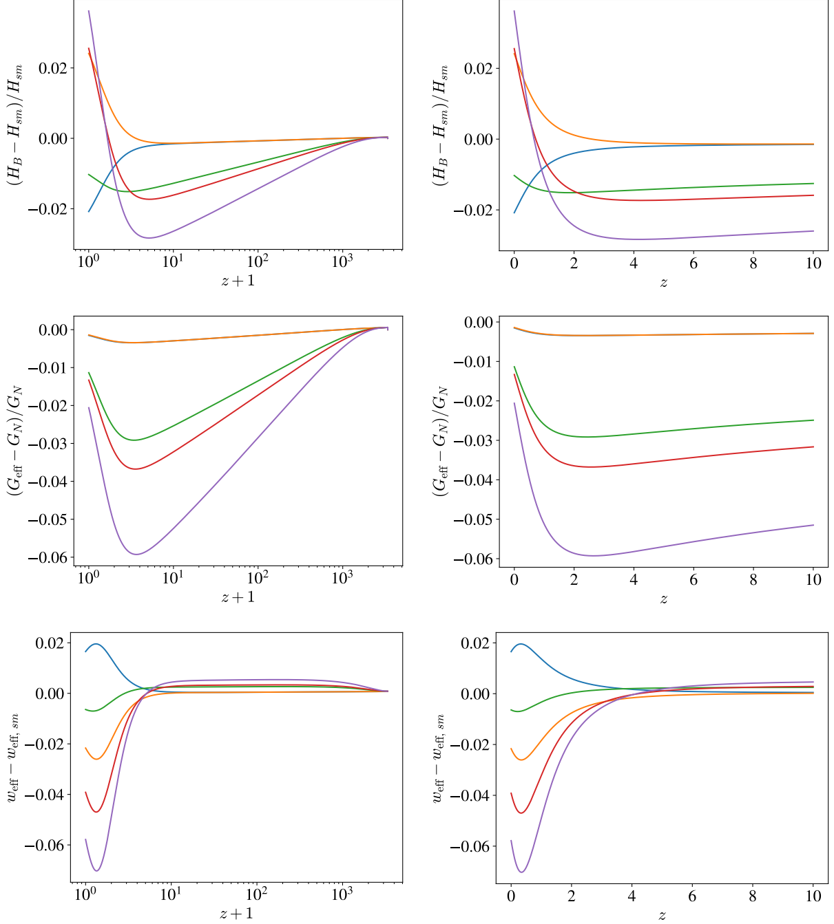
FIG. 6: Evolution of the cosmological quantities H_B , G_{\text{eff}} and w_{\text{eff}} as a function of the redshift in the baryon frame for \kappa = 10^{-3} and \epsilon_B = 10^{-3} . We zoom on the late evolution on the right. The values of \epsilon_C and \hat{\rho}_\Lambda for each colour are given in Fig.3.
