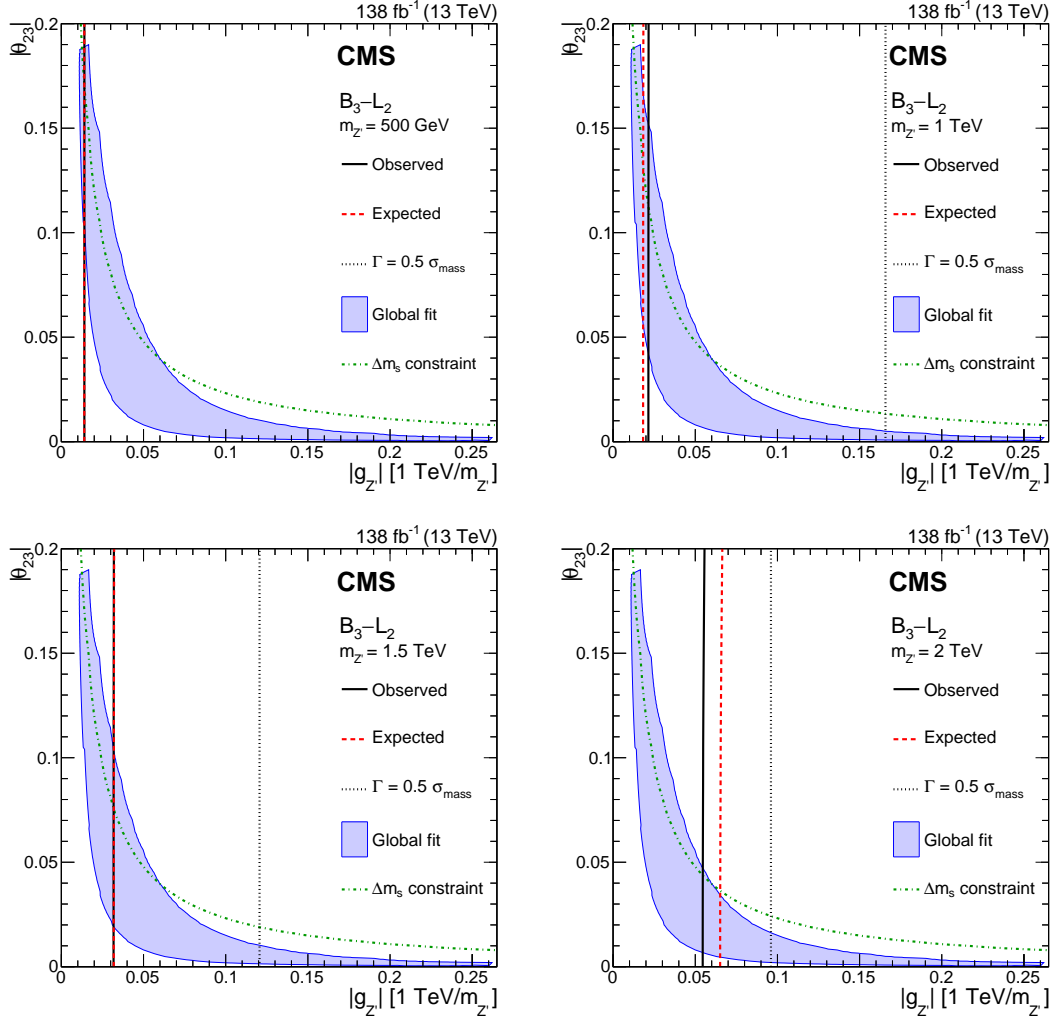
Figure 7: Exclusion limits at 95% CL in the |\theta_{23}| - |g_{Z'}| plane for the B_3-L_2 model [18], for representative values of m_{Z'} = 500 \text{ GeV} (upper left), m_{Z'} = 1 \text{ TeV} (upper right), m_{Z'} = 1.5 \text{ TeV} (lower left), and m_{Z'} = 2 \text{ TeV} (lower right). The solid black (dashed red) curves represent the observed (median expected) exclusions. The dotted curves denote the coupling values at which the Z' width equals one half of the \mu\mu invariant mass resolution. For larger values of the couplings, the narrow width approximation intrinsic to the search strategy is not considered valid. For a given mass, the region enclosed between the solid black (dashed red) and dotted curves is (expected to be) excluded. The dotted curve for m_{Z'} = 500 \text{ GeV} lies beyond the displayed |g_{Z'}| range and is, therefore, not shown. The shaded blue area represents the region preferred from the global fit in Ref. [18] at 95% CL. The region above the green dash-dotted curve is incompatible at 95% CL with the measurement of the mass difference between the mass eigenstates of the neutral B_s mesons [21].
