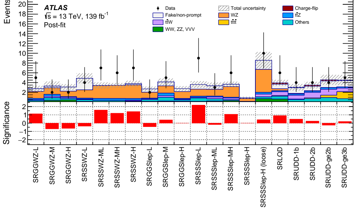
Figure 5: Data and post-fit background comparison in all SRs. The total uncertainties in the expected event yields are shown as the hatched bands. The bottom panel shows the significance [131] quantifying the deviation of the observed yields from the background expectation.
