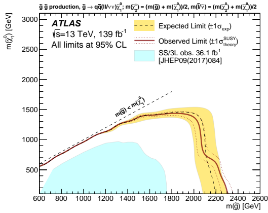
(c) \tilde{g} \rightarrow q\bar{q}(\ell\ell/\nu\nu)\tilde{\chi}_1^0
