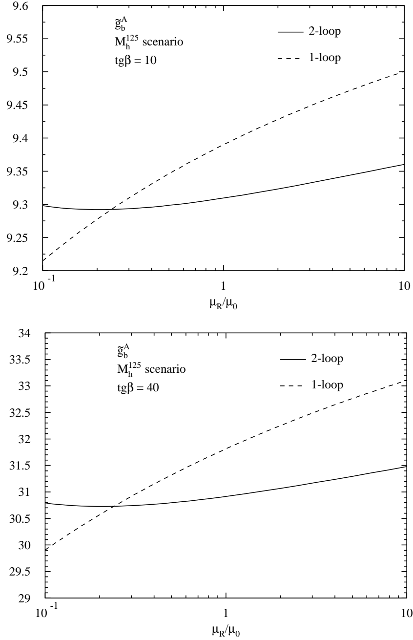
Figure 3: Scale dependence of the SUSY-QCD corrected effective Yukawa coupling factors \tilde{g}_b^A of Eq. (3) at one-loop and two-loop order in the M_h^{125} scenario as a function of the renormalization scale \mu_R and in units of the central scale choice \mu_0 = (m_{\tilde{b}_1} + m_{\tilde{b}_2} + m_{\tilde{g}})/3 . At leading order, g_b^A = 10(40) for \text{tg}\beta = 10(40) .
