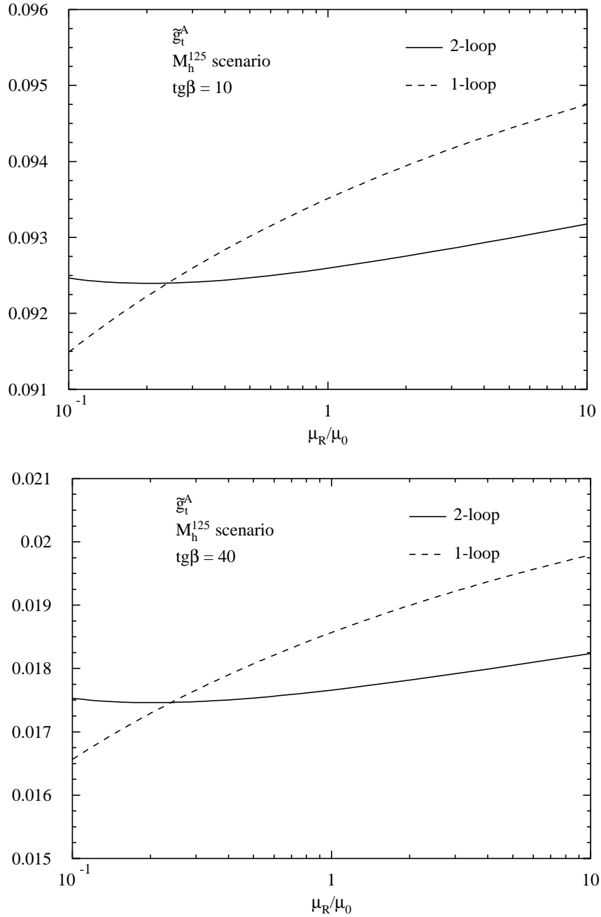
Figure 7: Scale dependence of the SUSY-QCD corrected effective Yukawa-coupling factors \tilde{g}_t^A at one-loop and two-loop order in the M_h^{125} scenario as a function of the renormalization scale \mu_R and in units of the central scale choice \mu_0 = (m_{\tilde{t}_1} + m_{\tilde{t}_2} + m_{\tilde{g}})/3 . At leading order, g_b^A = 0.1(0.025) for \text{tg}\beta = 10(40) .
