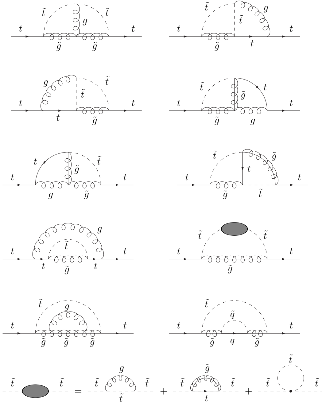
Figure 5: Two-loop diagrams of the SUSY-QCD contributions to the top self-energy involving top quarks t , top squarks \tilde{t} , gluons g and gluinos \tilde{g} . The squark-quark contributions to the gluino propagator have to be summed over all quark/squark flavors q/\tilde{q} , including both directions of the flavor flow due to the Majorana nature of the gluino.
