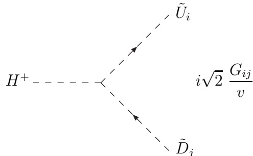
Figure 9: Feynman rule for the charged Higgs coupling to up- and down-type squarks, \tilde{U}_i and \tilde{D}_j ( ij = L, R or 1, 2 ), respectively.
