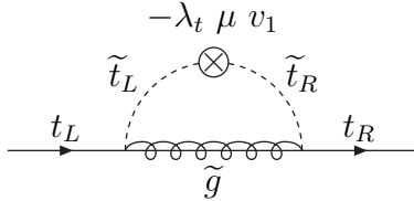
Figure 4: One-loop diagrams of the SUSY-QCD contributions to the top self-energy with the off-diagonal mass insertions corresponding to the corrections \Delta_t of the top Yukawa couplings. The contributing particles involve top quarks t , top squarks \tilde{t} and gluinos \tilde{g} .
