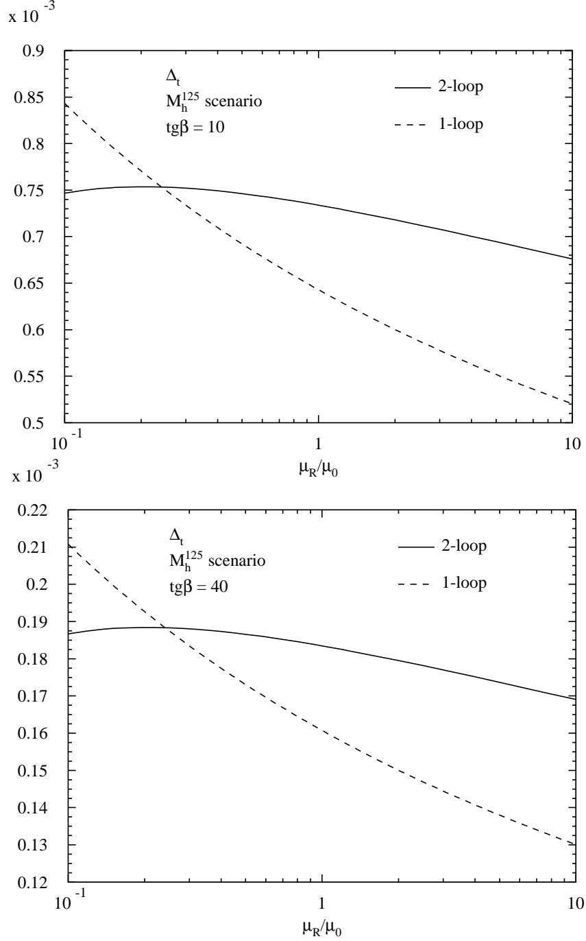
Figure 6: Scale dependence of the SUSY-QCD correction \Delta_t at one-loop and two-loop order in the M_h^{125} scenario for \text{tg}\beta = 10, 40 as a function of the renormalization scale \mu_R and in units of the central scale choice \mu_0 = (m_{\tilde{t}_1} + m_{\tilde{t}_2} + m_{\tilde{g}})/3 .
