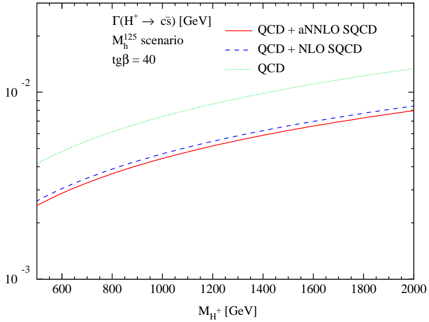
Figure 12: Same as Fig. 11 but for H^+ \rightarrow c\bar{b} (top) and H^+ \rightarrow c\bar{s} (bottom) for \text{tg}\beta = 40 .
