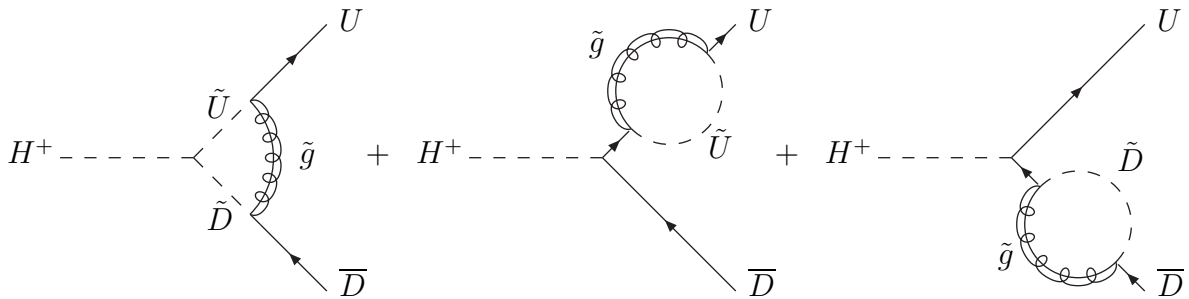
Figure 8: Virtual SUSY-QCD corrections to charged Higgs boson decays into U\bar{D} quark pairs at next-to-leading order. U denotes up-type and D down-type quarks.
