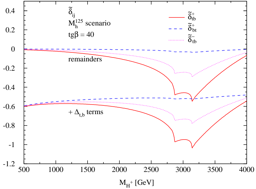
Figure 10: Individual NLO coefficients \tilde{\delta}_{ij}^{\pm} ( i, j = t, b ) of the decay width \Gamma(H^+ \rightarrow t\bar{b}) as a function of the charged Higgs mass with and without the \Delta_{t/b} contributions in the M_h^{125} scenario. The upper curves show the sizes of the SUSY-remainders, while the lower curves correspond to the full corrections including the \Delta_{t/b} contributions, without using the effective Yukawa couplings.
