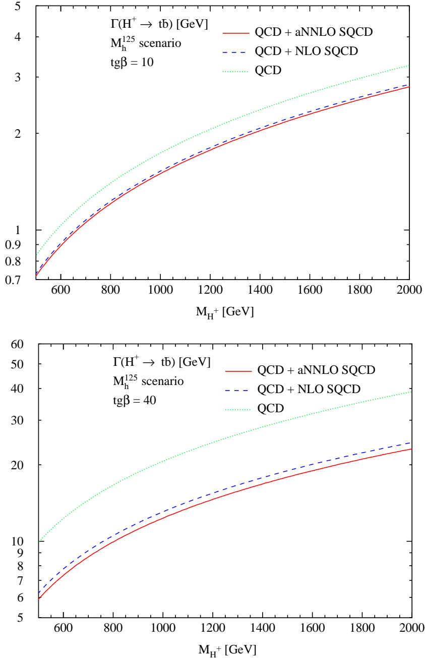
Figure 11: Partial decay width of H^+ \rightarrow t\bar{b} at different orders of the SUSY-QCD corrections. The dotted (green) lines include the usual QCD corrections involving the \overline{\text{MS}} Yukawa couplings, but no genuine SUSY-QCD corrections. The dashed (blue) lines involve the full NLO SUSY-QCD remainders in addition to the effective Yukawa couplings that have been used at the 1-loop level in SUSY-QCD. The full (red) lines display the approximate results (aNNLO) including the 2-loop SUSY-QCD corrections to the effective Yukawa couplings.
