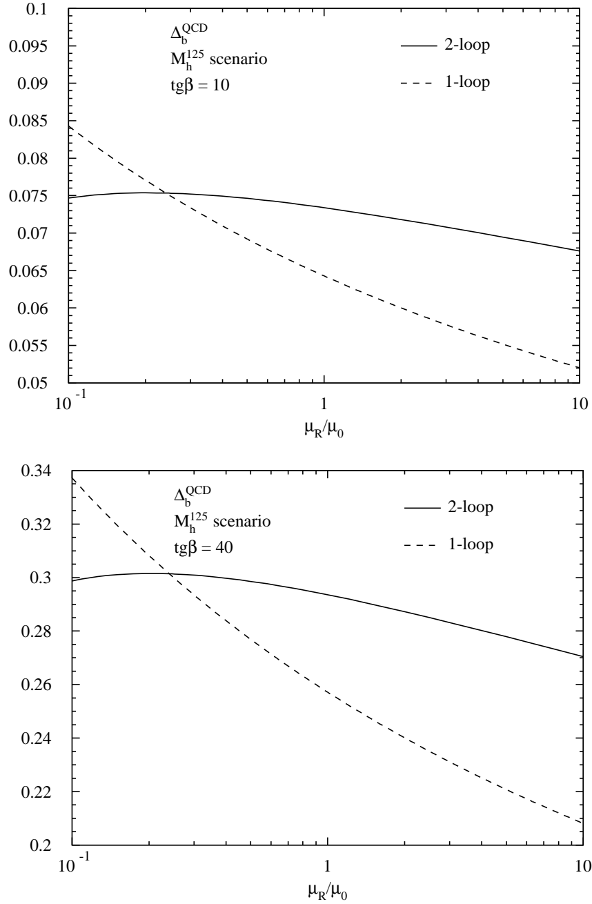
Figure 2: Scale dependence of the SUSY-QCD correction \Delta_b^{QCD} given in Eq. (4) at one-loop and two-loop order in the M_h^{125} scenario for \text{tg}\beta = 10, 40 as a function of the renormalization scale \mu_R and in units of the central scale choice \mu_0 = (m_{\tilde{b}_1} + m_{\tilde{b}_2} + m_{\tilde{g}})/3 .
