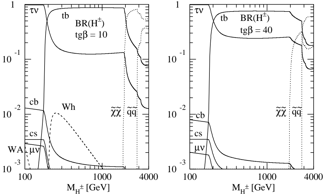
Figure 1: Branching ratios of the charged Higgs boson within the M_h^{125} scenario as a function of the charged Higgs mass for two values of \text{tg}\beta = 10, 40 . The results shown here include the results of this paper. The branching ratios into charginos and neutralinos ( \tilde{\chi}\tilde{\chi} ) involve the sum over all gaugino final states, whereas those into squarks ( \tilde{q}\tilde{q} ) incorporate the sum over all squark final states. This figure has been obtained with Hdecay [19].
