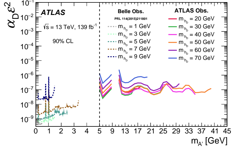
Figure 4: Observed 90% CL upper limits on \alpha_D \varepsilon^2 , as a function of m_{A'} with different dark Higgs boson masses, from this search (solid curves) compared with the results from Belle [15] (dashed curves).
