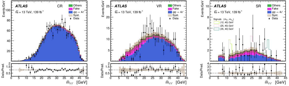
Figure 2: The \bar{m}_{\ell\ell} distribution in the CR, VR, and SR for the data and post-fit background contributions. The error bands include experimental and theoretical systematic uncertainties as constrained by a background-only fit. The contributions from the production of qq \rightarrow 4\ell events are scaled by a normalization factor 0.95, from the simultaneous fit in the SR and CR. The “Others” category combines gg \rightarrow ZZ , Higgs, VVV and t\bar{t}Z background contributions. The “Fake” background represents the contribution from non-prompt leptons. Three representative signal distributions are overlaid in the SR, assuming m_{h_D} = 40 GeV and different values of m_{A'} . The cross-sections for these benchmark points are calculated with \alpha_D = 0.1 and \varepsilon = 10^{-3} .
