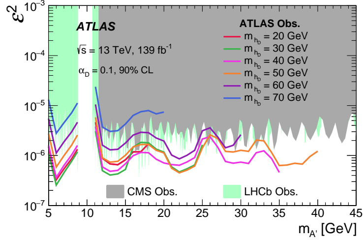
Figure 5: Observed 90% CL upper limits on \varepsilon^2 , assuming of \alpha_D = 0.1 , as a function of m_{A'} with different dark Higgs boson masses ranging from 20 GeV to 70 GeV. The parameter space excluded by LHCb [12] (CMS [77]) is covered by the green (gray) shaded regions.
