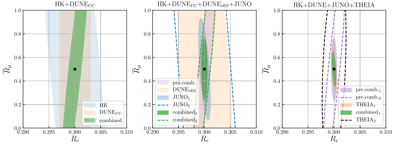
Fig. 3. The capability of next-generation neutrino detectors for measuring solar neutrino flavor compositions. The subscripts 1, 2 indicate that JUNO 1,2 and/or THEIA 1,2 is included in the analysis—see text for details. All contours are at 1\sigma CL and the assumed true value is marked by \star .
