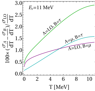
Fig. 2. Comparison between the differential cross sections, normalized to the leading order one (see Eq. (1)). In particular, we would like to draw reader's attention to the cyan line that demonstrates \mathcal{O}(1\%) difference between \nu_\mu and \nu_\tau scattering cross sections. This is the effect our phenomenological study is based on.
