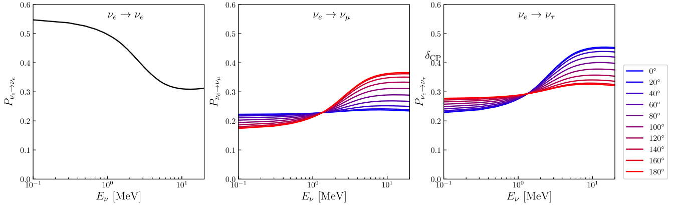
Fig. 4. The solar neutrino transition probabilities P_{\nu_e \rightarrow \nu_{\alpha}}(E_{\nu}) for various values of \delta_{\text{CP}} .
