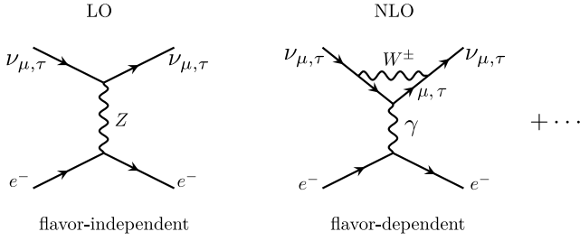
Fig. 1. Feynman diagrams for \nu_{\mu,\tau} scattering on electrons. The diagram on the left shows the leading order contribution whereas the one on the right illustrates the flavor-dependent NLO contribution.
