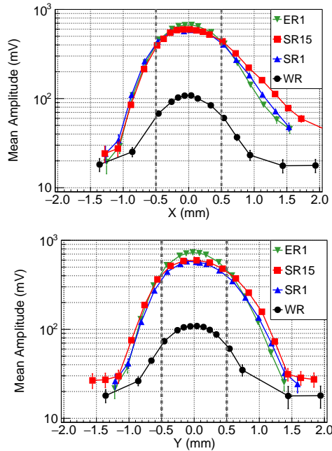
Fig. 2: Measured average signal as a function of the x (above) and y (below) with the position of the maximum setting the zero in the abscissa. The scans were performed at 3 V OV. The vertical dashed lines indicate the dimension of the SiPM.
