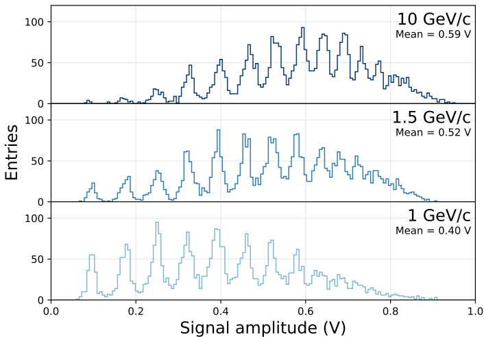
Fig. 5: Distribution of the detected number of SPADs for sensor SR1 at 10.0, 1.5 and 1.0 GeV/c. The plots are obtained at 3 V OV and with an oscilloscope vertical scale at 200 mV/div.
