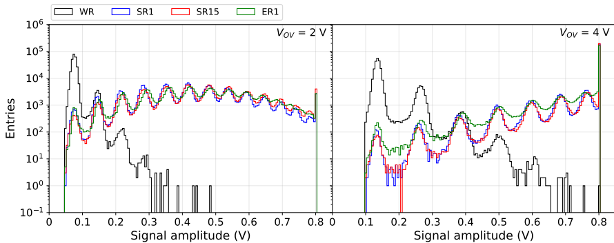
Fig. 3: Distribution of the amplitude for different sensors as measured at the position of the maximum signal average at OV (left) 2 V and (right) 4 V. The curves are obtained with an oscilloscope vertical scale at 100 mV/div. The plots are normalized to the same number of events.
