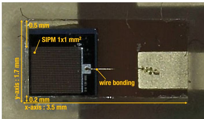
Fig. 1: Photograph of the SiPM sensor with the area covered by the protection layer. Notice that in the test beam, the dimensions 1.7 \text{ mm} \times 3.5 \text{ mm} correspond to the y and x coordinates, respectively.
