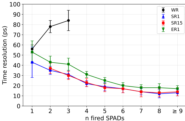
Fig. 7: Measured time resolution as a function of the number n of firing SPADs for the sensors described in Section 2 at 4 V OV. The last value of WR is intended to be for signals with \geq 3 SPADs firing.
