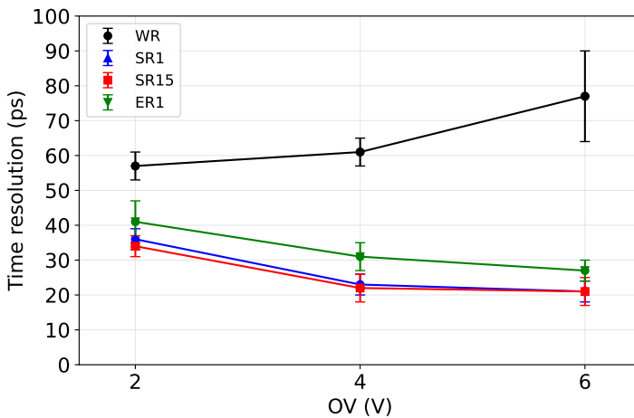
Fig. 6: Measured time resolution as a function of the over-voltage OV for the sensors described in Section 2.
