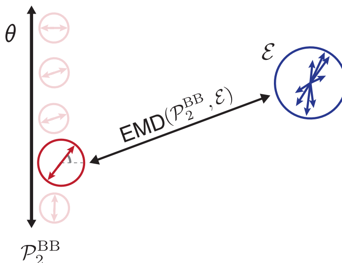
Figure 1. A representation of the EMD as the minimum distance of an event \mathcal{E} to a manifold of two-particle back-to-back events \mathcal{P}_2^{BB} . The angle \theta represents the degree of freedom corresponding to the relative azimuthal orientation of the reference event from \mathcal{P}_2^{BB} and the collider event \mathcal{E} . The arrow indicates, schematically, the EMD describing the minimum cost to transport \mathcal{E} to \mathcal{P}_2^{BB} .
