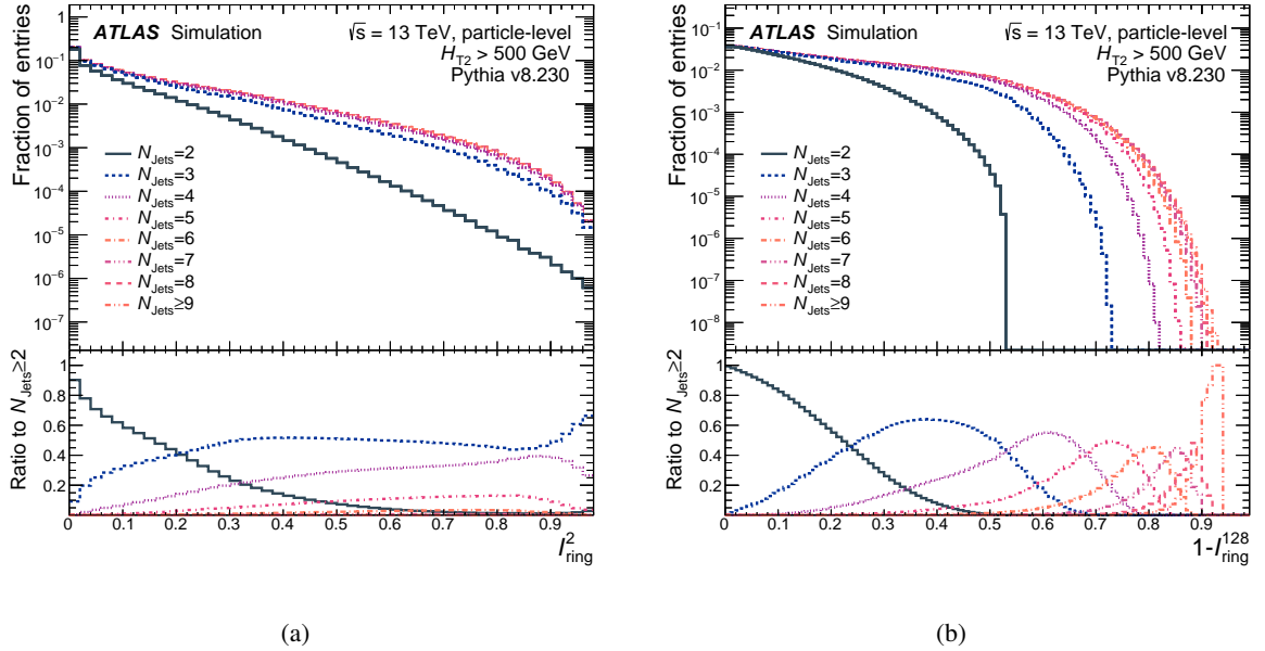
Figure 6: Stacked histograms show the normalised (a) \mathcal{I}_{\text{Ring}}^{N=2} and (b) 1 - \mathcal{I}_{\text{Ring}}^{N=128} distributions in separate bins of N_{\text{jet}} , for particle-level PYTHIA dijet events with N_{\text{jet}} \geq 2 and H_{T2} > 500 GeV. The lower panel of each figure shows the ratio of each N_{\text{jet}} bin to the inclusive distribution of the observable.
