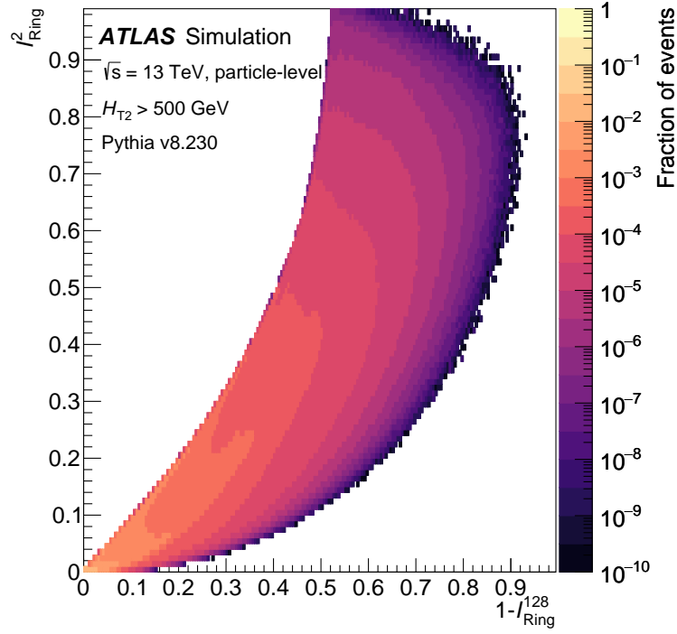
Figure 5: The correlation between \mathcal{I}_{\text{Ring}}^{N=2} and 1 - \mathcal{I}_{\text{Ring}}^{N=128} is illustrated as a two-dimensional histogram, for events with N_{\text{jet}} \geq 2 and H_{T2} > 500 GeV.
