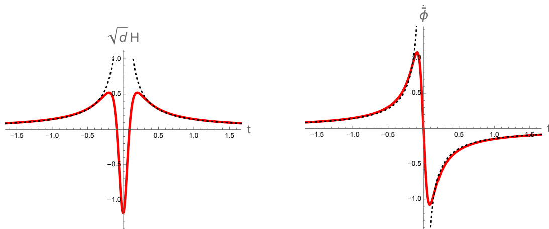
Figure 4. The time behaviour of the solution (2.8), (2.10) is represented by the solid red curves, plotted for d = 3 and \alpha' = 2 (for graphical reasons, we have expressed time in units of 5\sqrt{\alpha'} ). The dashed black curves describe the behaviour of the (singular) low-energy pre- and post-big bang branches, corresponding to the asymptotic limits t \rightarrow \mp\infty . The smooth transition between the initial accelerated to the final decelerated expansion is triggered by a high-curvature phase of accelerated/decelerated contraction.
