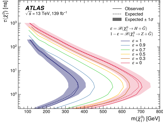
Figure 10: The 95% CL exclusion limits on the target signal hypothesis, for \tilde{\chi}_1^0 lifetime in ns as a function of \tilde{\chi}_1^0 mass in GeV. The overlaid curves correspond to different decay hypotheses, where the assumed cross-section is for higgsino production, and the \tilde{\chi}_1^0 decays to H + \tilde{G} or Z + \tilde{G} such that \mathcal{B}(H + \tilde{G}) + \mathcal{B}(Z + \tilde{G}) = 100\% . The curve shown in red represents the decay hypothesis where the \tilde{\chi}_1^0 decays to Z + \tilde{G} with 100% branching ratio. The curve shown in blue represents the decay hypothesis where the \tilde{\chi}_1^0 decays to H + \tilde{G} with 100% branching ratio.
