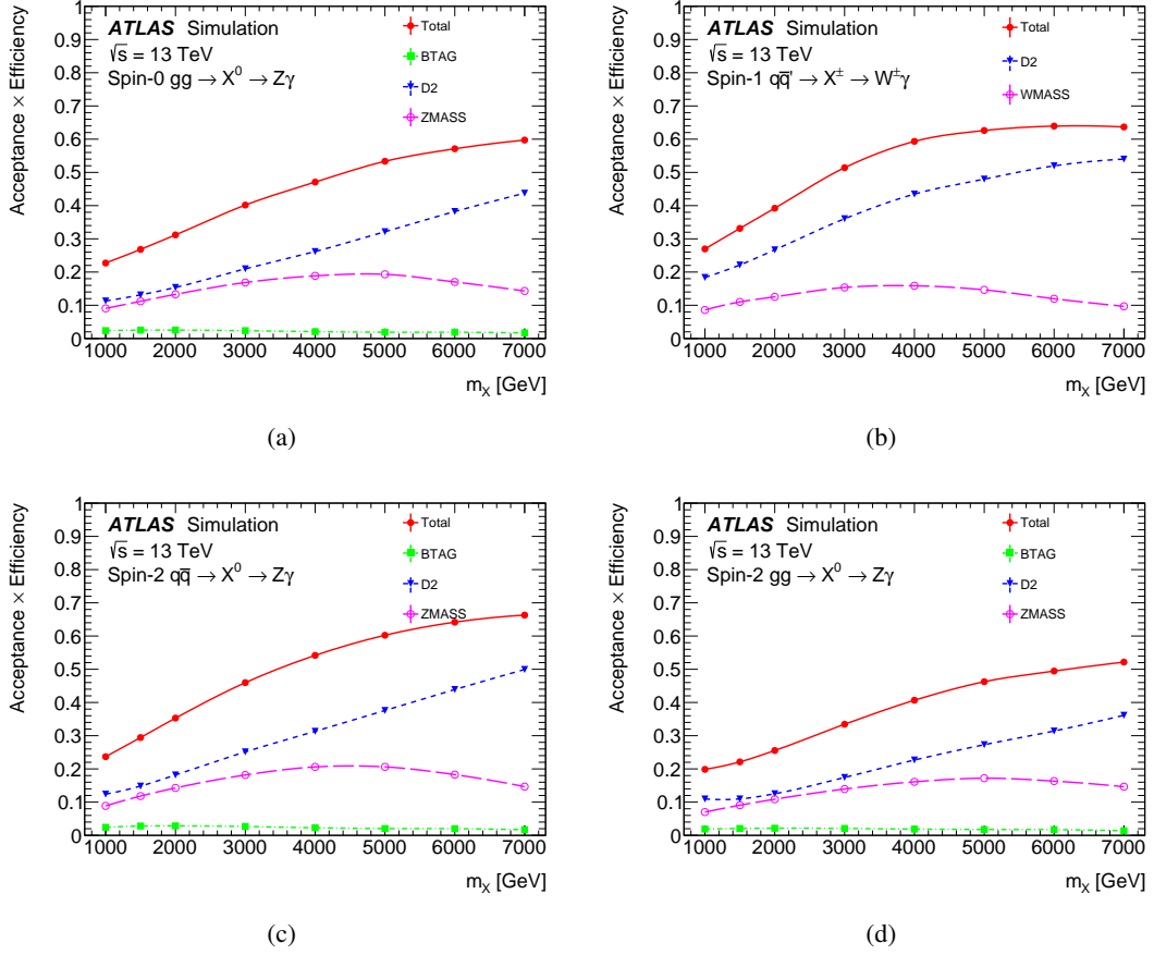
Figure 3: Total efficiencies for the selection of signal events after categorization and application of the tighter photon E_T^\gamma selection used to optimize the signal significance: (a) spin-0 gg \rightarrow X^0 \rightarrow Z\gamma , (b) spin-1 q\bar{q} \rightarrow X^\pm \rightarrow W^\pm\gamma , (c) spin-2 q\bar{q} \rightarrow X^0 \rightarrow Z\gamma , and (d) spin-2 gg \rightarrow X^0 \rightarrow Z\gamma . In addition to the total efficiency, contributions to the signal selection from each of the separate event categories are shown. The efficiencies calculated from MC samples with W/Z hadronic decays are shown as the points on each curve. The line presents interpolated results.
