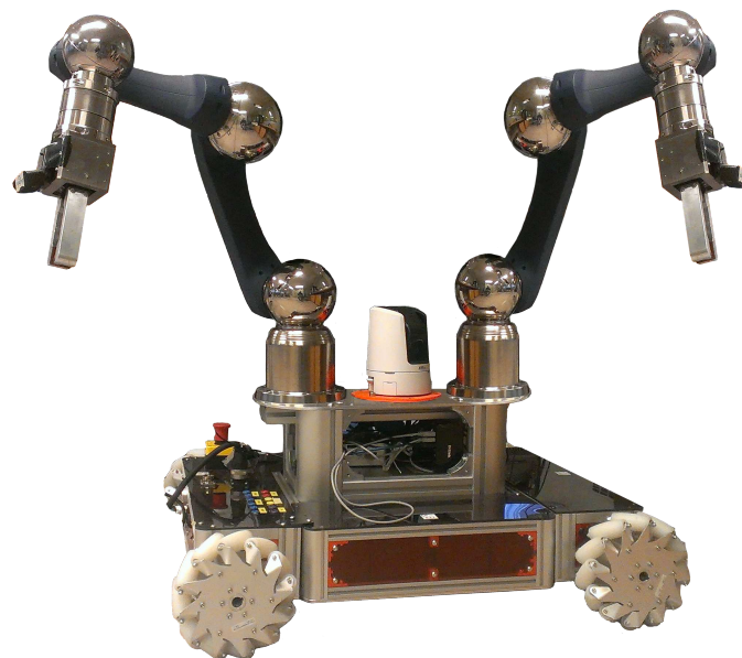
Figure 1. Dual-arm CERNBot.
