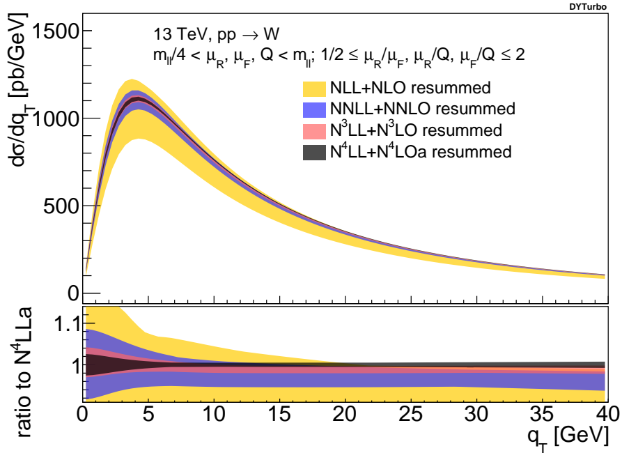
Figure 2: The q_T spectrum of W^+ and W^- bosons with inclusive leptonic decay at the LHC ( \sqrt{s} = 13 TeV) at various perturbative orders. Resummed component (see Eq. (7)) of the hadronic cross-section with scale variation bands as defined in the text.
