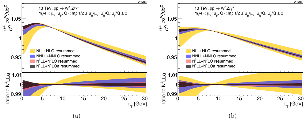
Figure 3: The normalized ratio of q_T spectra of W and Z/\gamma^* bosons at the LHC ( \sqrt{s} = 13 TeV) at various perturbative orders for W^+/Z (left) and W^-/Z (right). Resummed component (see Eq. (7)) of the hadronic cross-section with scale variation bands as defined in the text.
