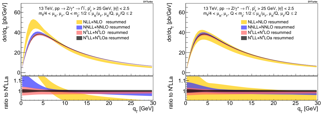
Figure 1: The q_T spectrum of Z/\gamma^* bosons with lepton selection cuts at the LHC ( \sqrt{s} = 13 TeV) at various perturbative orders. Resummed component (see Eq. (7)) of the hadronic cross-section with scale variation bands as defined in the text. The order of the parton density evolution is set consistently with the order of the resummation (left) or with the order of the PDFs (right).
