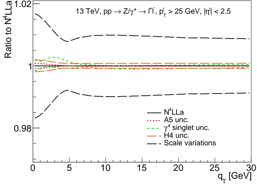
Figure 4: Uncertainties arising from numerical approximations or incomplete knowledge of the perturbative coefficients at N^4LL+N^4LOa , compared to missing higher order uncertainties estimated with scale variations at this order.
