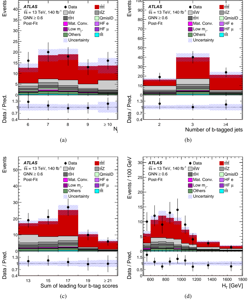
Figure 6: Comparison between data and prediction after the fit to data in the signal-enriched region with GNN \geq 0.6 for the distributions of (a) the number of jets, (b) the number of b -jets, (c) the sum of the four highest PCBT scores of jets in the event, and (d) the sum of transverse momenta over all jets and leptons in the event ( H_T ). The ratio of the data to the total post-fit computation is shown in the lower panel. The shaded band represents the total post-fit uncertainty in the prediction. The first and last bins contain underflow and overflow events, respectively.
