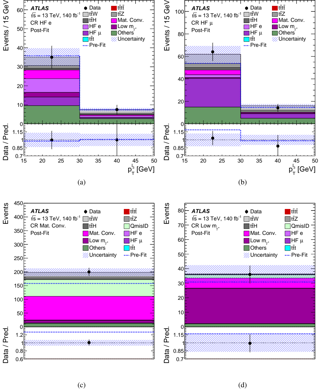
Figure 4: Post-fit distributions for the fitted variables in the CRs for the fake/non-prompt lepton background. For (a) CR HF e and (b) CR HF μ, the third-highest lepton p_T is fitted, while for (c) CR Mat. Conv. and (d) CR Low m_{\gamma^*} , the number of events is used. The ratio of the data to the total post-fit prediction is shown in the lower panel. The dashed blue lines show the pre-fit prediction in the upper panel and the ratio of the data to the total pre-fit prediction in the lower panel. The shaded band represents the total post-fit uncertainty in the prediction. In (a) and (b), the last bin contains the overflow.
