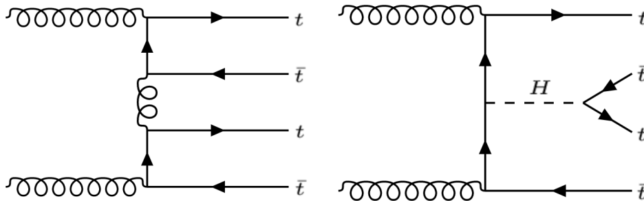
Figure 1: Illustrative tree-level Feynman diagrams for the SM t\bar{t}t\bar{t} signal. The mediator connecting two top quarks can be a gluon, a neutral electroweak gauge boson ( \gamma or Z ), or a Higgs boson.
