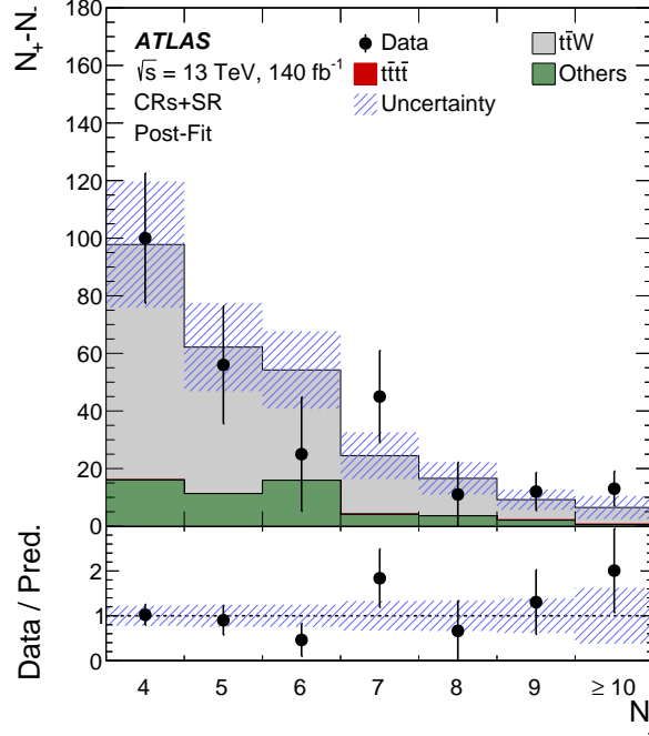
Figure 3: Post-fit distribution for the difference between the number of positive events and the number of negative events ( N_+ - N_- ) as a function of the number of jets ( N_j ) in the sum of four t\bar{t}W CRs and the SR. The uncertainties on the normalisation factors and on the t\bar{t}W modelling parameters are represented by the shaded band. The ratio of the data to the total post-fit prediction is shown in the lower panel.
