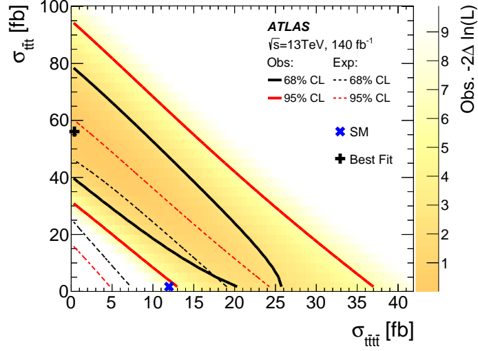
Figure 7: Two-dimensional negative log-likelihood contour for the t\bar{t} cross section ( \sigma_{t\bar{t}} ) versus the t\bar{t}t\bar{t} cross section ( \sigma_{t\bar{t}t\bar{t}} ) when the normalisation of both processes are treated as free parameters in the fit. The blue cross shows the SM expectation of \sigma_{t\bar{t}t\bar{t}} = 12 fb from Ref. [16] and \sigma_{t\bar{t}} = 1.67 fb (see Section 3), both computed at NLO, while the black cross shows the best-fit value. The observed (expected) exclusion contours at 68% (black) and 95% CL (red) are shown in solid (dashed) lines. The gradient-shaded area represents the observed likelihood value as a function of \sigma_{t\bar{t}} and \sigma_{t\bar{t}t\bar{t}} .
