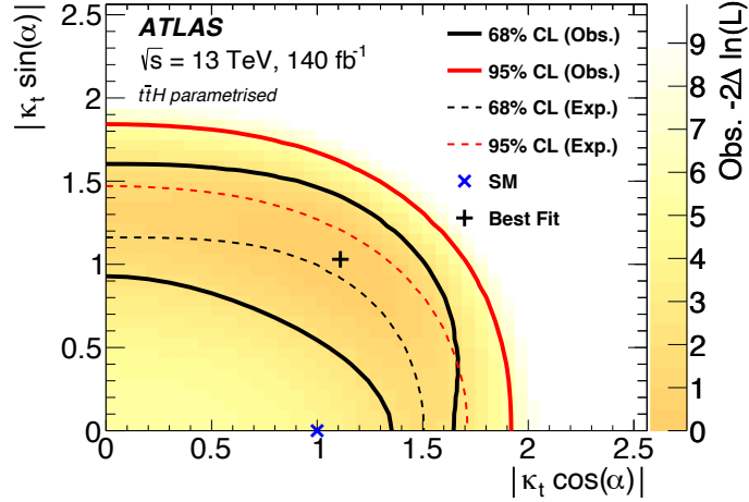
Figure 8: Two-dimensional negative log-likelihood contours for |\kappa_t \cos(\alpha)| versus |\kappa_t \sin(\alpha)| at 68% and 95%, where \kappa_t is the top-Higgs Yukawa coupling strength parameter and \alpha is the mixing angle between the CP -even and CP -odd components. The gradient-shaded area represents the observed likelihood value as a function of \kappa_t and \alpha . Both the t\bar{t}t\bar{t} signal and t\bar{t}H background yields in each fitted bin are parameterised as a function of \kappa_t and \alpha . The blue cross shows the SM expectation, while the black cross shows the best fit value.
