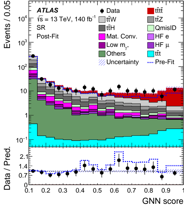
Figure 5: Comparison between data and the predictions after a fit to data for the GNN distribution in the SR. The first bin contains underflow events. The ratio of the data to the total post-fit prediction is shown in the lower panel. The dashed blue lines show the pre-fit prediction in the upper panel and the ratio of the data to the total pre-fit prediction in the lower panel. The shaded band represents the total post-fit uncertainty in the prediction.
