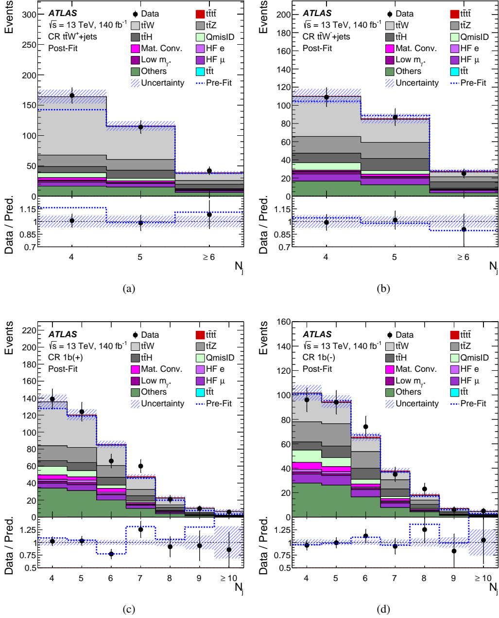
Figure 2: Post-fit distributions for the number of jets ( N_j ) in each of the four t\bar{t}W CRs: (a) CR t\bar{t}W^+ +jets, (b) CR t\bar{t}W^- +jets, (c) CR 1b(+) and (d) CR 1b(-). The ratio of the data to the total post-fit prediction is shown in the lower panel. The dashed blue lines show the pre-fit prediction in the upper panel and the ratio of the data to the total pre-fit prediction in the lower panel. The shaded band represents the total post-fit uncertainty in the prediction.
