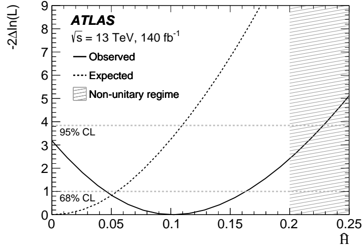
Figure 9: The negative log-likelihood values as a function of the Higgs oblique parameter \hat{H} . The solid line represents the observed likelihood while the dashed line corresponds to the expected one. The dashed region shows the non-unitary regime.
