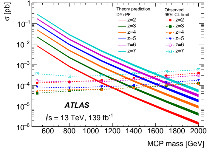
Figure 8: Observed 95% CL cross-section upper limits and theoretical cross-sections as functions of the muon-like spin- \frac{1}{2} MCP's mass for the DY+PF production mode. Theoretical cross-section values are computed at LO and the uncertainty bands correspond to the PDF uncertainties.
