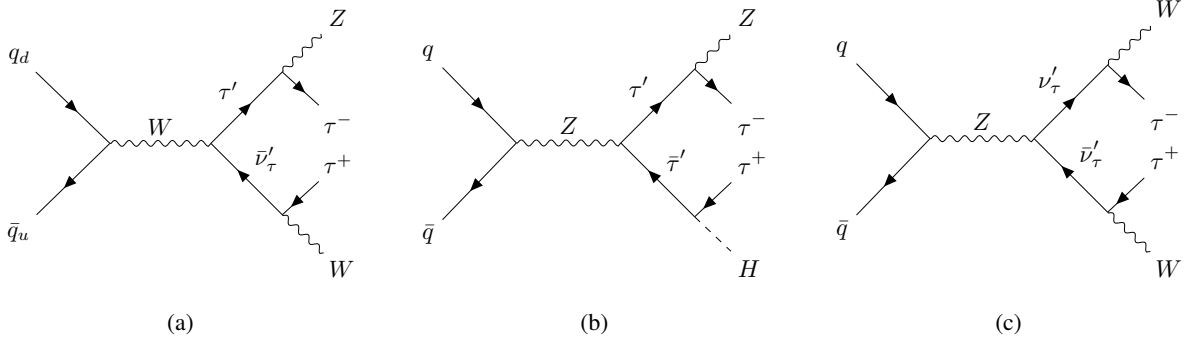
Figure 1: Examples of LO Feynman diagrams for VLL production and decay: (a) \tau' \bar{\nu}'_{\tau} production followed by \tau' decay into Z\tau^- and \bar{\nu}'_{\tau} decay into \tau^+W^- , where q_u ( q_d ) represents a weak isospin +1/2 ( -1/2 ) quark, (b) production of \tau' \bar{\tau}' followed by the decay into Z\tau^- and \tau^+H , and (c) \nu'_{\tau} \bar{\nu}'_{\tau} production followed by \nu'_{\tau} decay into W\tau^- .
