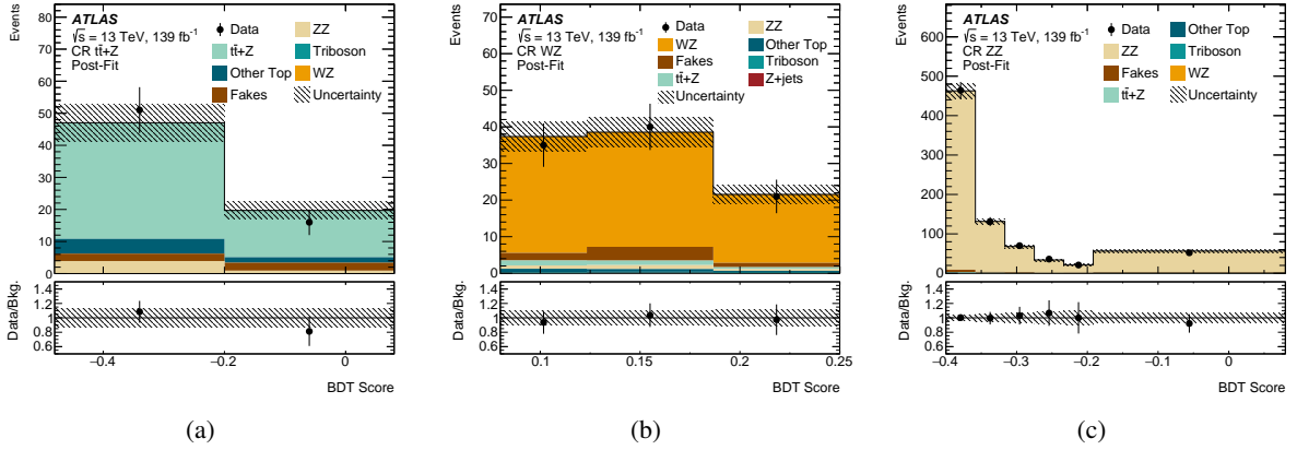
Figure 2: A comparison of the BDT scores for data and the predicted background after performing the fit described in Section 8 in the CRs used to estimate the three dominant backgrounds: (a) t\bar{t}+Z , (b) WZ , and (c) ZZ . The first bin of the t\bar{t}+Z and ZZ distributions contains underflow events, while the last bin of the WZ distribution contains overflow events. The hatched band represents the combined statistical and systematic uncertainties.
