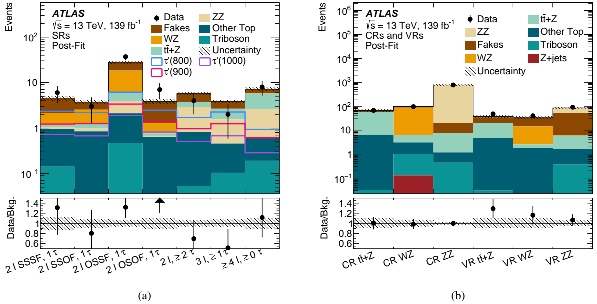
Figure 4: Summary of post-fit yields for data and background, and pre-fit yields for signal modelling in the (a) SRs and (b) CRs and corresponding VRs. Uncertainty bands contain both the systematic and statistical uncertainties post-fit. Background normalization factors are also applied. The ‘Other Top’ sample includes contributions from single top, t\bar{t} , t\bar{t}+W , t+Z , t+WZ , t\bar{t}+H , t\bar{t}+WW , t\bar{t}t\bar{t} , and ttt . The arrow in the ratio plot is for the point that is outside the range.
