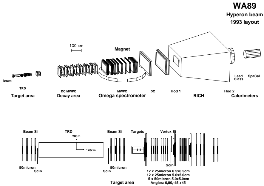
Figure 1: WA89 experimental set-up in 1993
