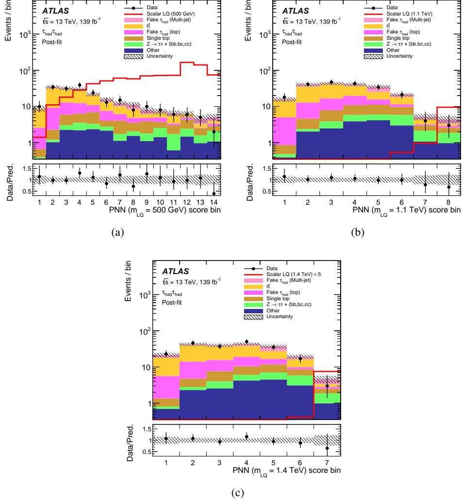
Figure 8: The PNN score distributions in the \tau_{\text{had}}\tau_{\text{had}} SR for (a) m_{LQ} = 500 GeV, (b) m_{LQ} = 1.1 TeV, (c) m_{LQ} = 1.4 TeV. The normalisation and shape of the backgrounds are determined from the background-only likelihood fit to data and the ratios of the data to the sum of the backgrounds are shown in the lower panels. ‘Other’ refers to the sum of minor backgrounds (vector boson + jets, diboson and Higgs boson). The hatched bands indicate the combined statistical and systematic uncertainty in the total background predictions. The expected signals for scalar LQs with the corresponding masses, scaled by the indicated factors for visibility, are overlaid. Since the PNN score itself is not a physical quantity, it is represented solely by the bin number.
