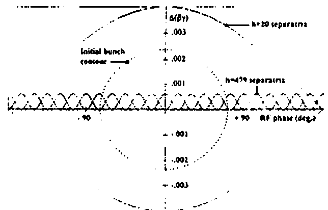
Figure 4: Longitudinal phase space during the production of flat-topped bunches.
