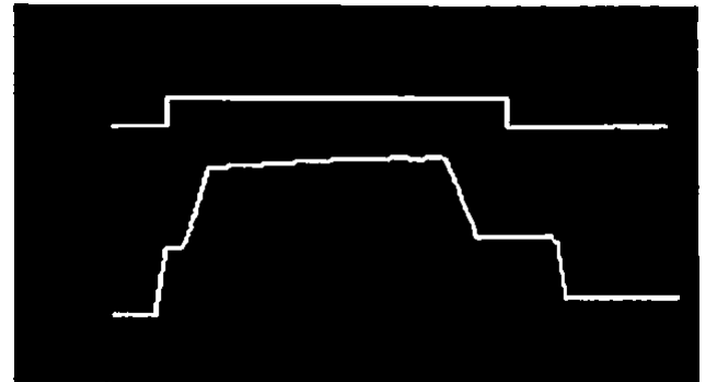
Figure 1: Beam current ( 2 \times 10^{12} protons/div.) and RF voltage (50 kV/div.) versus time (200 ms/div.).
