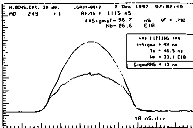
Figure 5: Quasi-parabolic bunch. The dotted curve is a Gaussian fit to the 1-D density profile (upper trace). The lower trace is the 2-D phase space density derived from the profile by an Abel transform [8].
