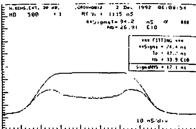
Figure 6: Flat-topped bunch. The Abel transform reveals the depopulation at low synchrotron amplitude.
