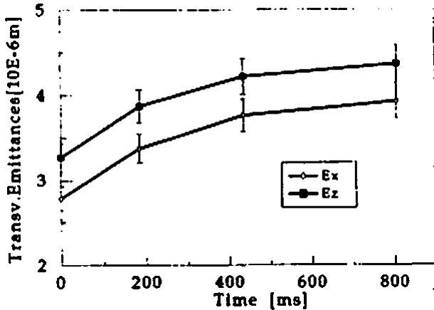
Figure 3: Transverse emittances, \mathcal{E}_{x,s} , versus time in a strong space charge regime ( |\Delta Q_{x,s}| = 0.45 ) at 1 GeV with Q_{x,s} = 6.22, 6.28 . Injection is at t = 0 .
