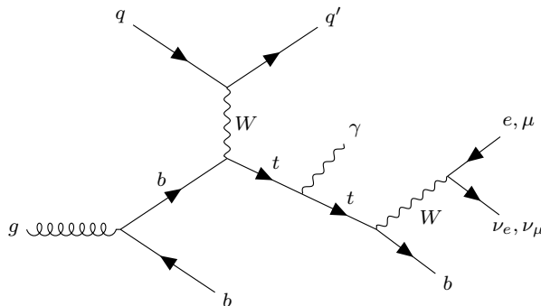
Figure 1: Representative Feynman diagram at leading order in \alpha_s for tq\gamma production with semileptonic top-quark decay.
