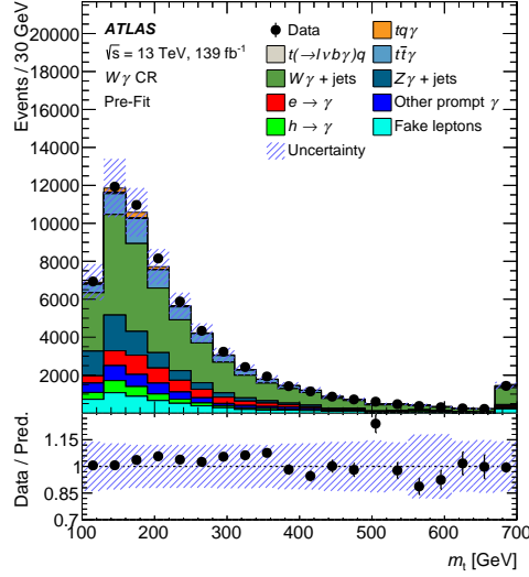
Figure 2: Distribution of the reconstructed top-quark mass in the W\gamma CR before the profile-likelihood fit. The hashed band represents the uncertainties and the first and last bins include the underflow and overflow.
