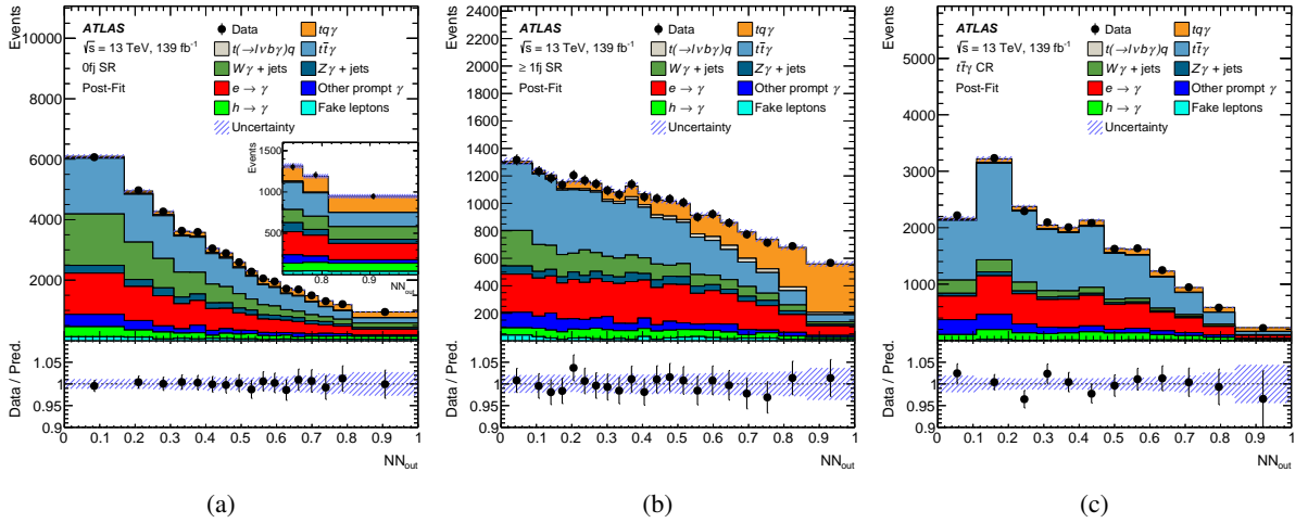
Figure 3: Distributions of the NN outputs in (a) the 0fj SR, (b) the \geq 1 fj SR, and (c) the t\bar{t}\gamma CR in data and the expected contribution of the signal and background processes after the profile-likelihood fit. The hashed band represents the uncertainties in the SM prediction. The inset in (a) presents a close-up of the last three bins of the NN output.
