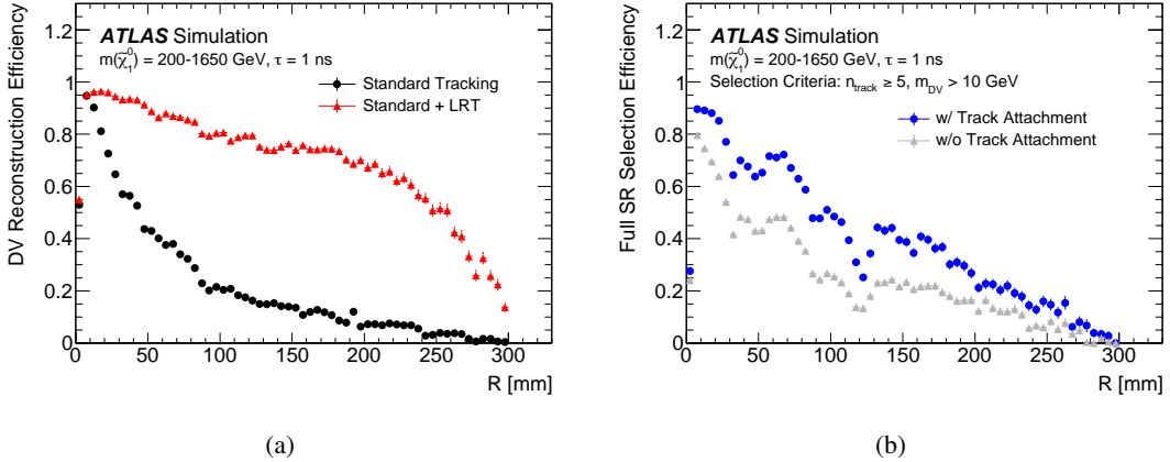
Figure 2: In (a), the DV reconstruction efficiencies with and without the special LRT processing are shown for a combined sample of simulated Strong RPV and EWK RPV events with m(\tilde{g}) = 1.8-2.2 TeV, m(\tilde{\chi}_1^0) = 200-1650 GeV and \tau(\tilde{\chi}_1^0) = 1.0 ns. The efficiency is defined as the probability for a true neutralino decay with at least two charged decay products with p_T > 1 GeV and |\eta| < 5 to be matched with a reconstructed DV. In (b), the impact of attached tracks on the total SR selection efficiency of the same combined sample is shown. The total SR selection efficiency is defined in Section 5.
