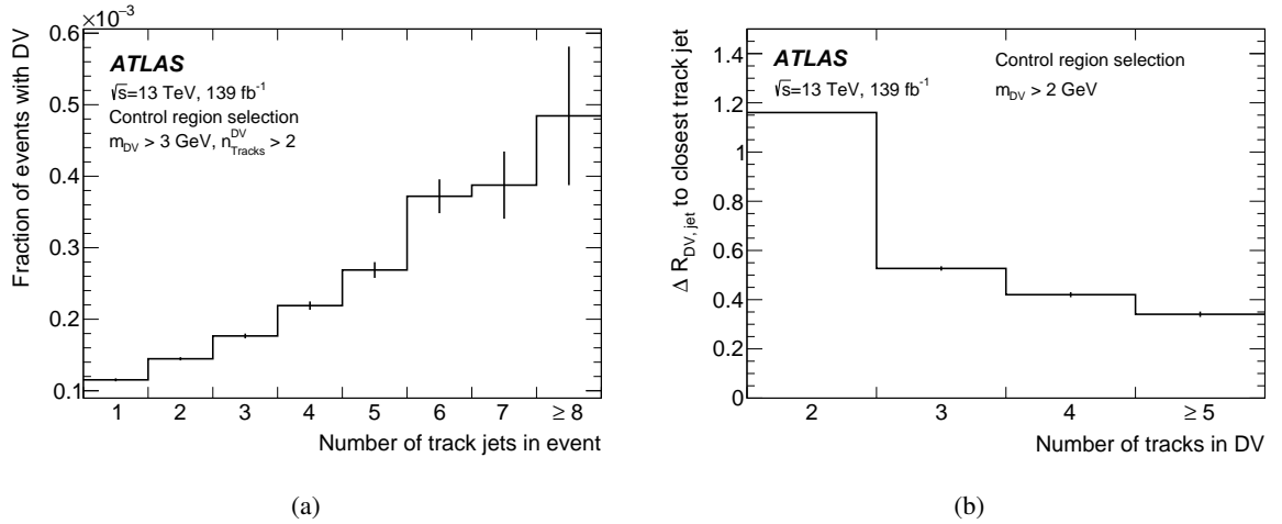
Figure 4: In (a), the fraction of events in the CR with a reconstructed DV satisfying m_{\text{DV}} > 3 GeV and n_{\text{Tracks}}^{\text{DV}} > 2 is shown. In (b), the average distance of DVs with m_{\text{DV}} > 2 GeV to the closest track jet in the event is shown, as a function of n_{\text{Tracks}} .
