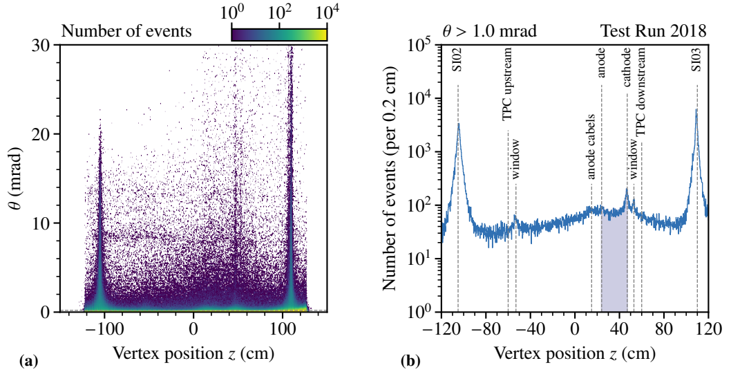
Figure 2.19: The scattering angle dependence on the vertex z -position is shown in (a). In (b) the vertex z -position is shown for scattering angles \theta > 1 mrad. No selection of the cathode beam hole as well as the vertex z -positions are applied to visualize the different structures. In blue the active area of the TPC is indicated.
