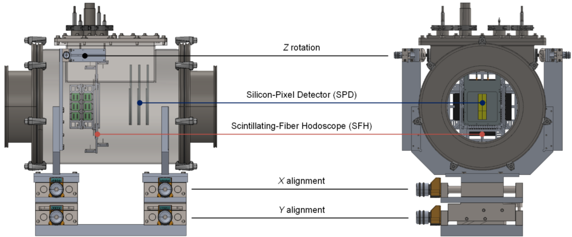
Figure 1.16: Technical drawing of the UTS. The SPD and SFH detector planes are indicated as well as the positioning system for the alignment. Figure taken from [41].
