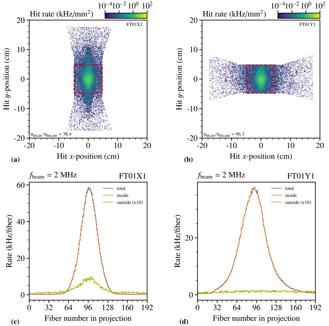
Figure A.4: Fiber hit positions and rate for the x- and y-projection of the FT01 station. In (a) and (b) the respective position with the central 96 \times 96 \text{ mm}^2 area marked in red. The overall ratio between inner and outer hits is given in the figure. In (c) and (d) the corresponding rates per channel are shown. The different contributions between the inner and outer part.
