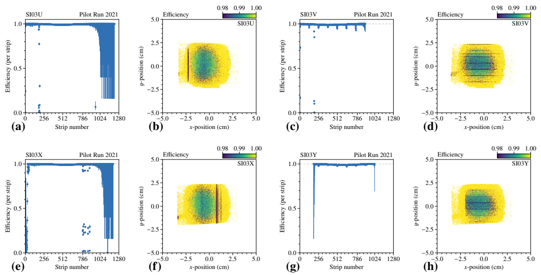
Figure D.4: Silicon efficiencies in 1-d and 2-d projection for SI03.
