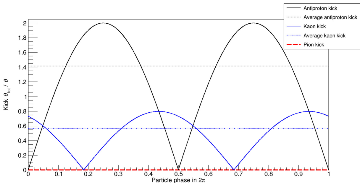
Fig. 6. Illustration of deflection of pions, antiprotons and kaons for \Delta\theta_{\text{pion}}^{\text{antiproton}} = \pi .
