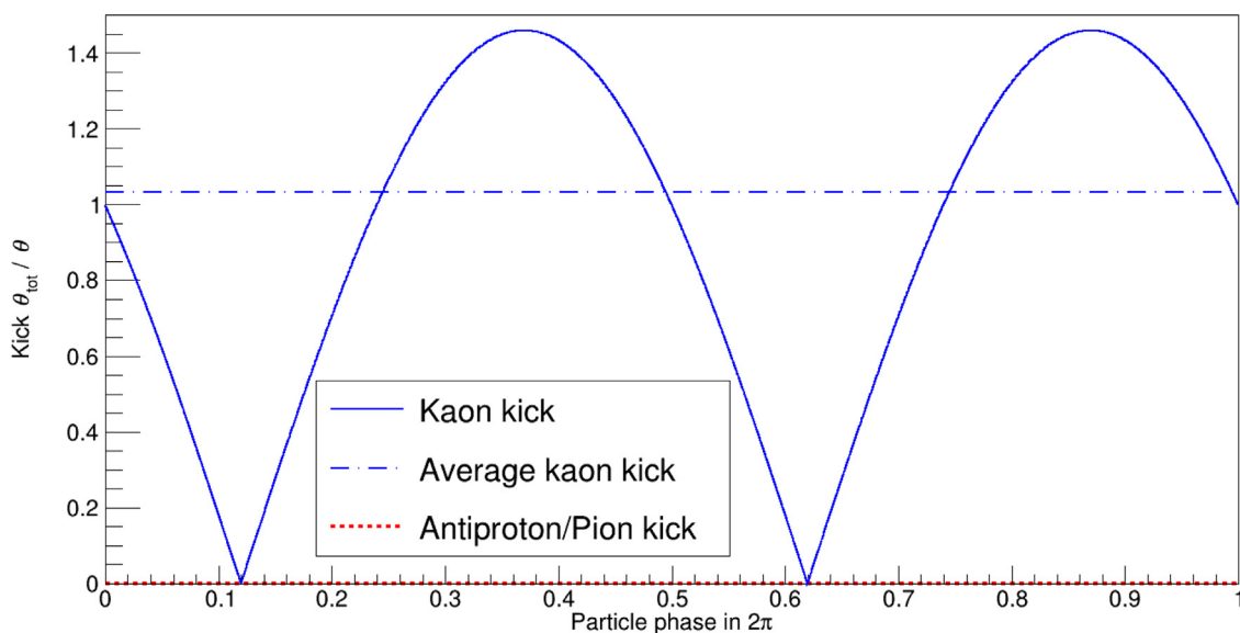
Fig. 5. Illustration of deflection of pions, antiprotons and kaons for \Delta\varphi_{\text{pion}}^{\text{antiproton}} = 2\pi .
