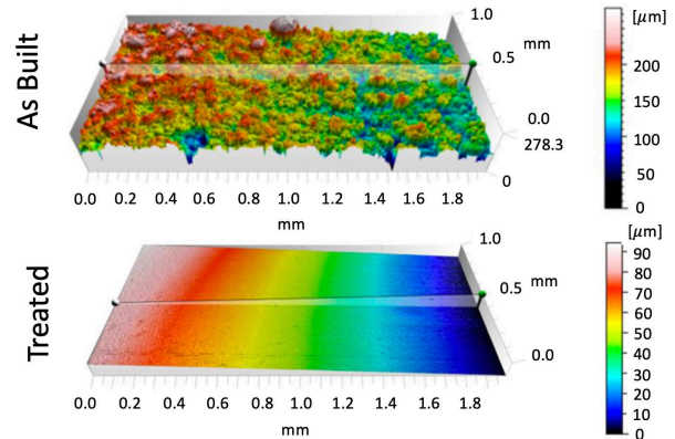
Figure 7: 3D surface roughness of the post-processed ¼ RFQ sample.
