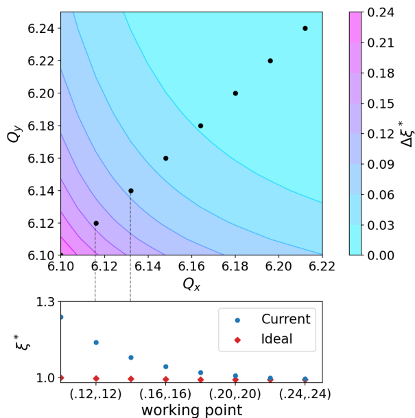
Figure 1: \xi^* for both current and ideal configurations when the working point is moved closer to the integer resonance, with \Delta\xi^* being the difference between both configurations.
