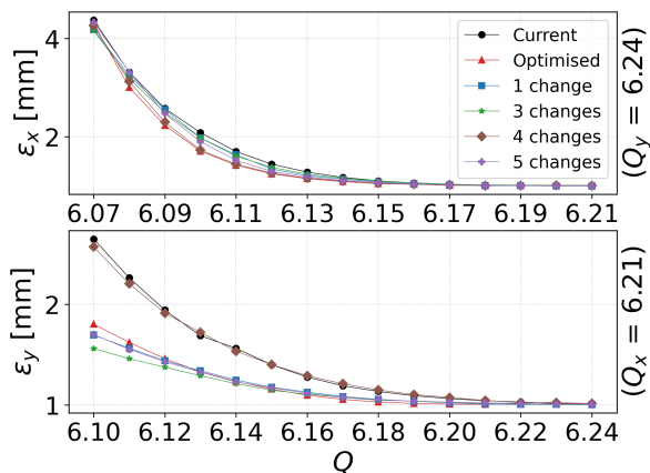
Figure 2: Evolution of the normalised emittances 5 ms after injection obtained with space-charge simulations using different quadrupole configurations.
