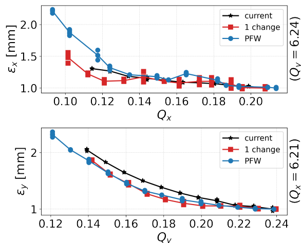
Figure 3: Experimental results of the tunes scans for the current PS lattice performed using the LEQs, the PFWs and the 1-change configuration. The scans are performed with WS 64V and 65H.
