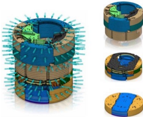
Figure 2: ESS Target Inner Shielding.
