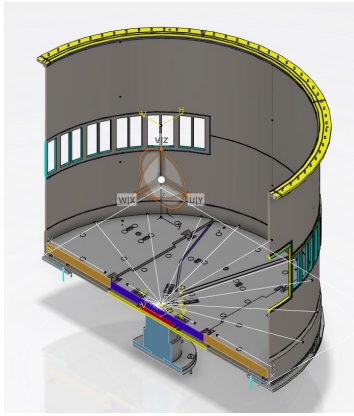
Figure 1: ESS Target Vessel Inner Shielding First Layer.
