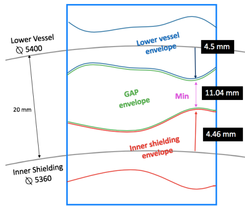
Figure 4: Inner Shielding First Layer Gap Reduction Results.
