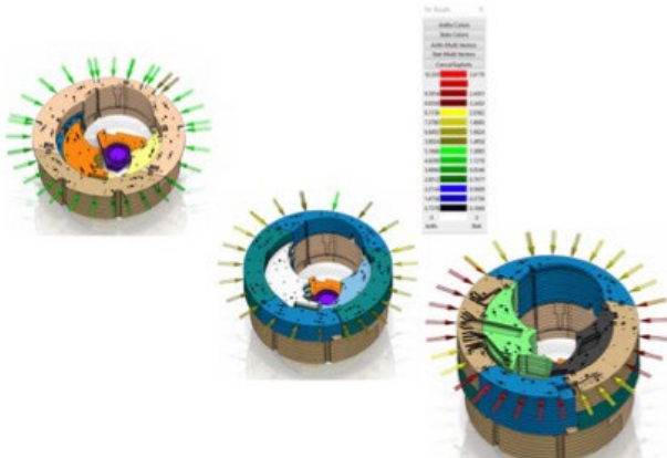
Figure 5: Inner Shielding Gap Reduction Results.
