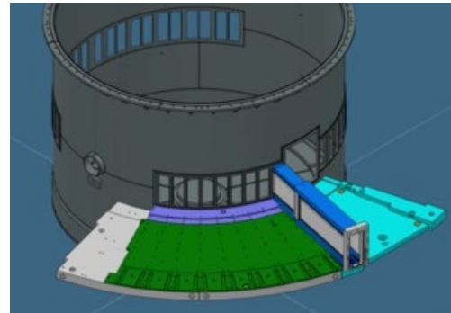
Figure 3: ESS Target Port Tube Assembly.
