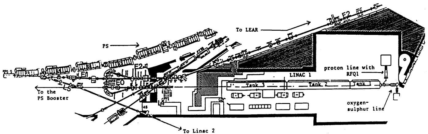
Figure 2. The Linac Layout in 1992
