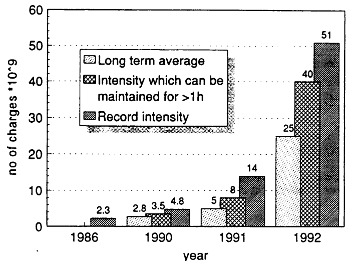
Figure 3. Progression of sulphur charges in the PS supercycle (sum of 4 pulses).
