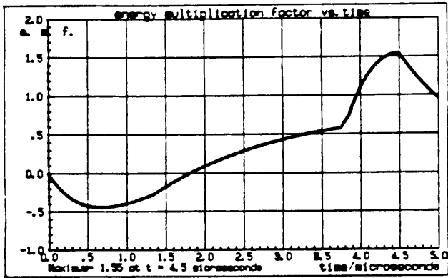
Fig. 5 Energy multiplication factor versus time
