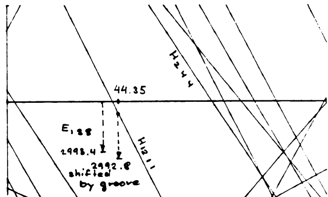
Fig. 2 Investigated mode: H 0 3 8 at 2998.55 MHz Vertical scale from 2988.55 to 3008.55 MHz Horizontal scale from 44.00 to 45.00 cm
