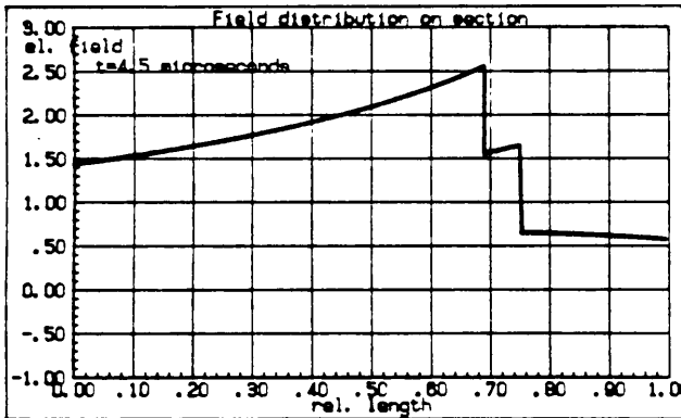
Fig. 6 Field distribution on the accelerating section
