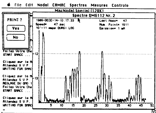
Fig 4 - Spectral gas analysis
