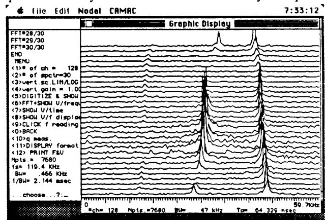
Fig 3 - Onset of betatron e- beam instabilities
