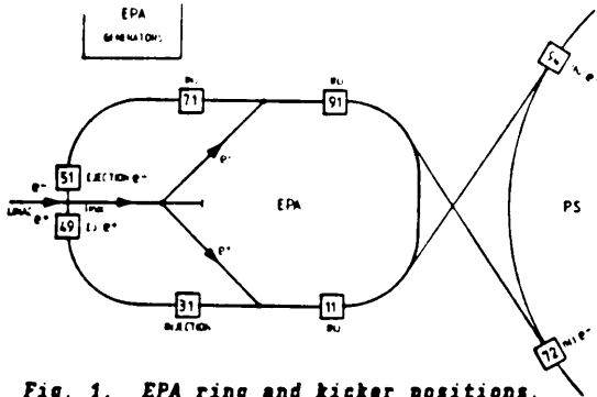
Fig. 1. EPA ring and kicker positions.
