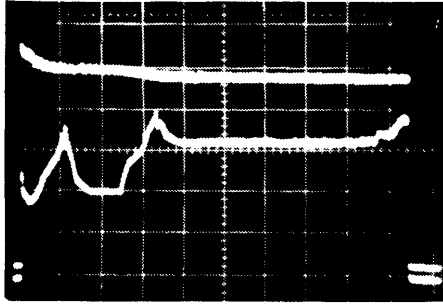
Fig. 7: Beam current (top) and peak-detected wide-band PU for the entire acceleration cycle (100 ms/div.). First loss during and after merging, a few % loss at transition (second peak in bottom trace).
