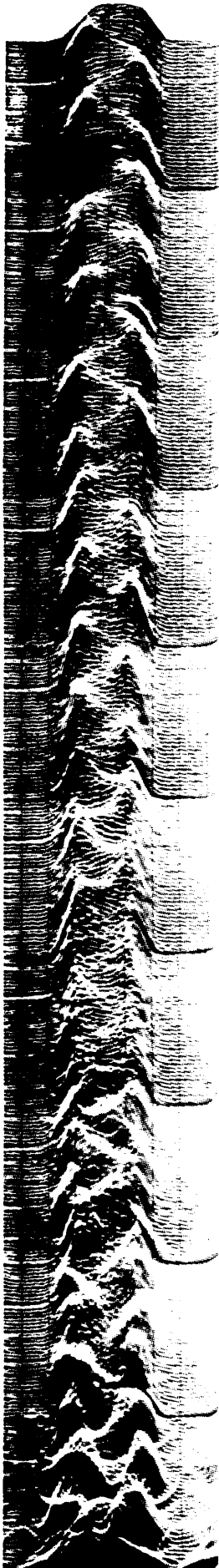
Fig. 3: Mountain-range display of the first 10 ms of merging in the PS of two bunches from the PSB. Horizontal sweep, 20 ms/division. Only every tenth turn is displayed. The time goes from bottom to top.
