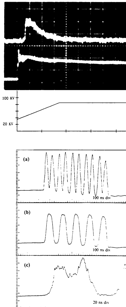
Fig. 5: Top trace: Amplitude of 1.4 GHz component of the longitudinal wide-band PU signal showing the onset of microwave instabilities 1 ms after injection. Bottom trace: Peak-detected signal of the same PU, representing peak line density. The trapping RF voltage program on the same time-scale (2 ms/div.) is plotted below.
