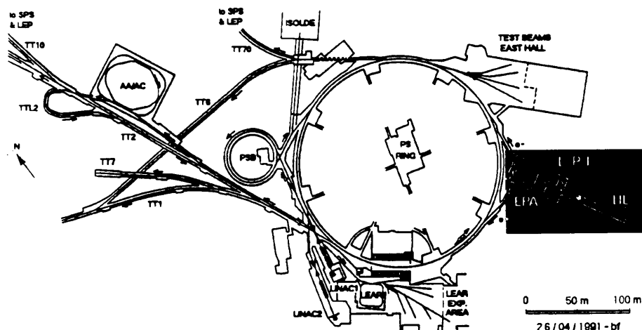
Figure 1. The CERN Proton Synchrotron (CPS) layout, with LPI accelerators highlighted
