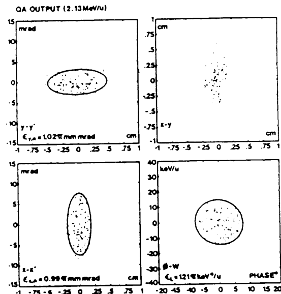
Figure 2: Phase Plane Projections at 2.13 MeV/u
