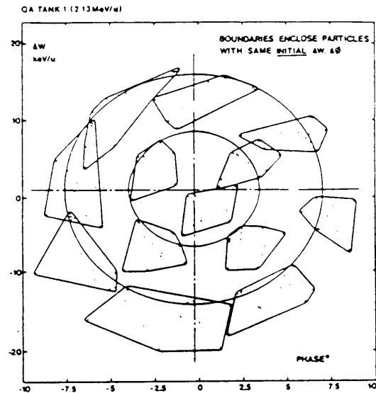
Figure 1: Coupling from Transverse to Longitudinal Phase Plane
