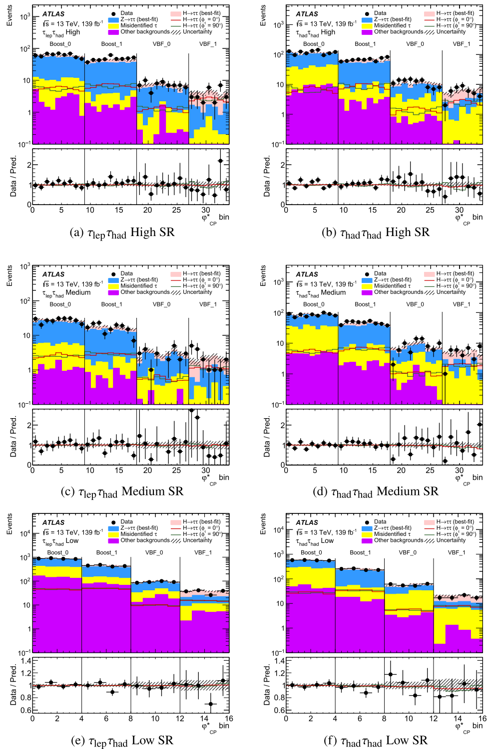
Fig. 4 Post-fit distributions of \phi_{CP}^* in the signal regions (SRs), showing a \tau_{lep} \tau_{had} High SR, b \tau_{had} \tau_{had} High SR, c \tau_{lep} \tau_{had} Medium SR, d \tau_{had} \tau_{had} Medium SR, e \tau_{lep} \tau_{had} Low SR, and f \tau_{had} \tau_{had} Low SR. The \phi_{CP}^* bins are counted incrementally through all VBF and Boost categories and cover the range [0, 360]^\circ for each category. The best-fit H \rightarrow \tau\tau signal is shown in solid pink, while the red and green lines indicate the predictions for the pure CP -even (scalar, SM) and pure CP -odd (pseudoscalar) hypotheses, respectively, scaled to the predicted signal yield. ‘Other backgrounds’ include W , diboson, top, Z \rightarrow \ell\ell and H \rightarrow WW^* . The hatched uncertainty band includes all sources of uncertainty after the fit to data
