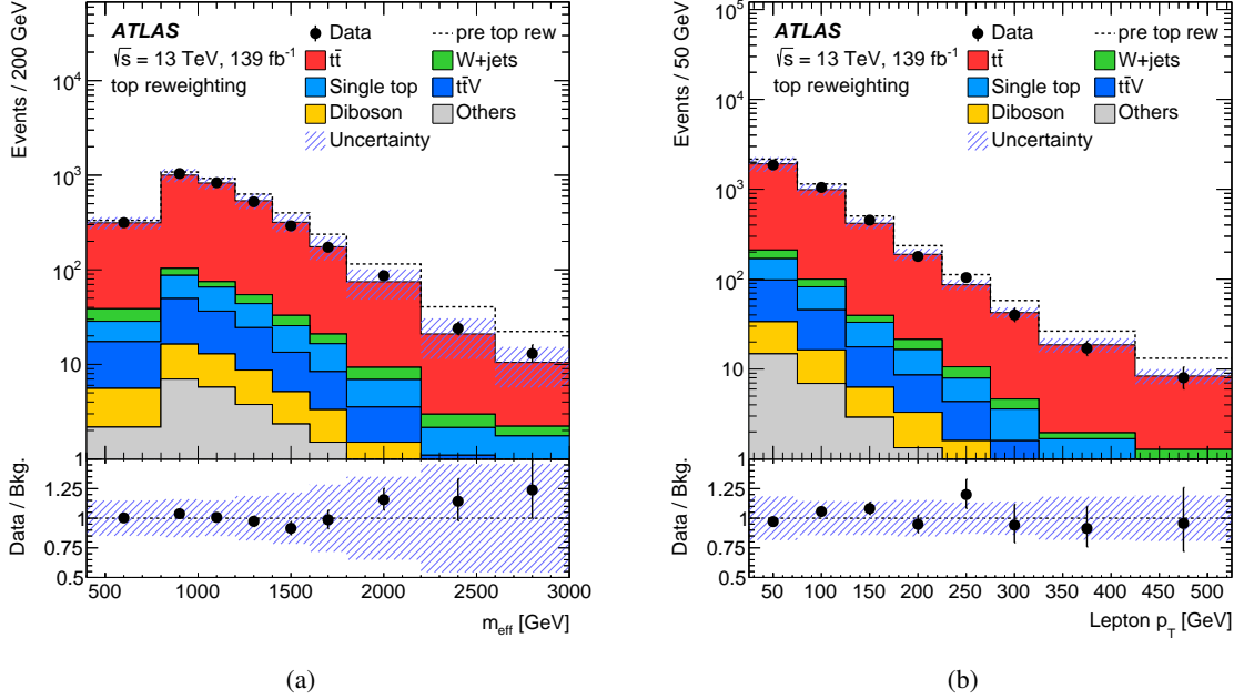
Figure 2: Distributions of (a) m_{\text{eff}} and (b) lepton p_T in the top reweighting region after applying the reweighting factors to the t\bar{t} and single-top background. The dashed line indicates the total background before the reweighting. The band includes statistical and systematic uncertainties. Minor background contributions from t\bar{t}H , tWZ , and Z +jets are combined into Others . The ratios of the data to the expected background are shown in the bottom panels of the plots. The last bin in each distribution contains the overflow.
