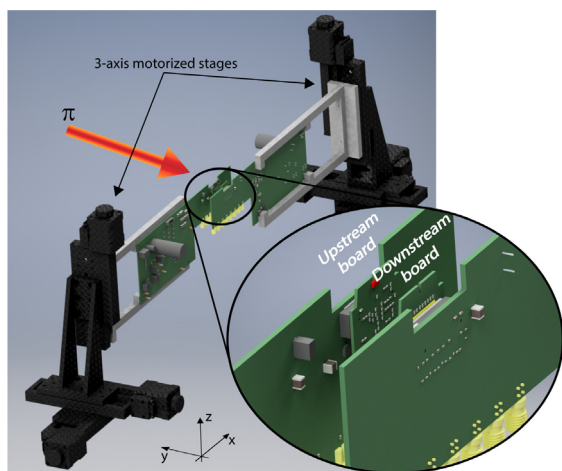
Fig. 2. Experimental MIP coincidence measurement setup.
