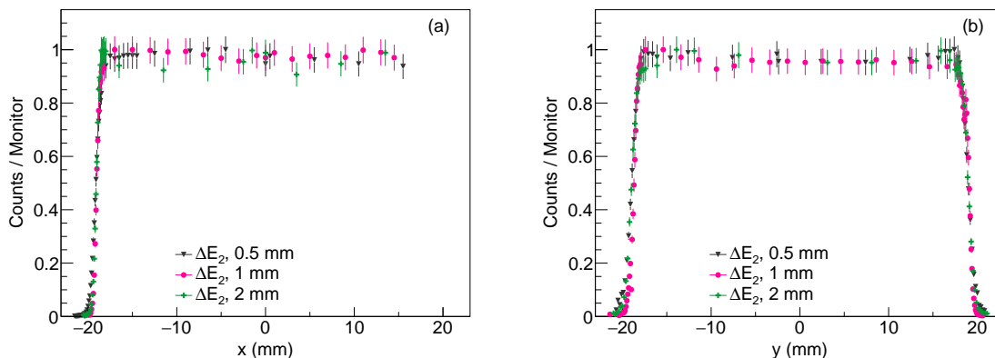
Figure 13. Measurements of the \Delta E_2 scintillator profiles performed at the PTB micro beam facility. The detectors have lateral dimensions of 38 mm \times 38 mm, and thickness of 0.5 mm, 1 mm, or 2 mm (as written in the figure). The x - y plane (the detector square face) was normal to the proton beam direction. The x -axis (panel (a)) corresponds to the axis of the PMT, with the PMT placed at x > 19 mm; the y -axis (panel (b)) is perpendicular to it. The measurements along the x -axis were not performed edge-to-edge but were stopped mid-way because otherwise the detector casing would have bumped against the beamline.
