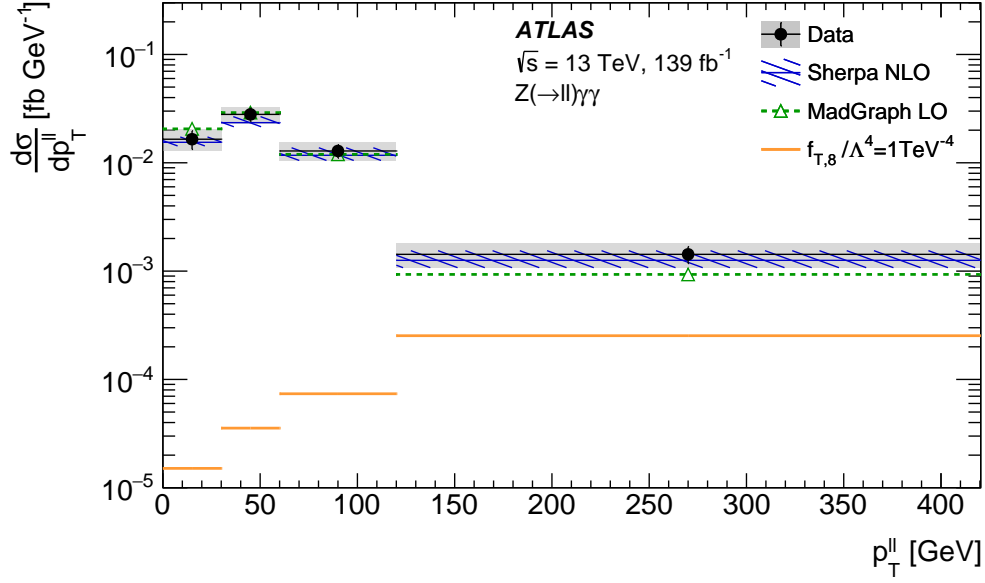
Figure 8: Comparison of the differential cross-section at particle level as a function of the dilepton transverse momentum between the observation in full Run 2 data, the NLO prediction from SHERPA, the LO prediction from MADGRAPH5_AMC@NLO, and the EFT prediction of one dimension-8 operator. The black uncertainty line on the data represents the statistical uncertainty, whereas the slightly taller grey uncertainty band represents the total uncertainty. The uncertainty in the SHERPA prediction includes both the statistical and theoretical uncertainties. The coupling parameter f_{T,8}/\Lambda^4 for the NP contribution of transverse operator \mathcal{O}_{T,8}^8 is set to 1/\text{TeV}^4 . The NP contribution contains interference effects between the SM Z\gamma\gamma production and the contribution of transverse operator \mathcal{O}_{T,8}^8 .
