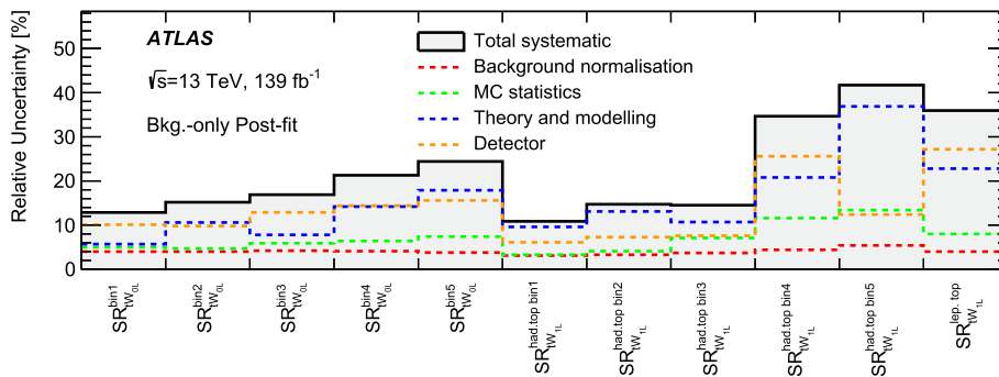
Fig. 6 Relative uncertainties (in percent) in the total background yield in each signal region of the two analysis channels, including the contributions from the different sources of uncertainty. The ‘Detector’ category contains all detector-related systematic uncertainties. The ‘Background normalization’ represents the uncertainty in the fitted normal-
