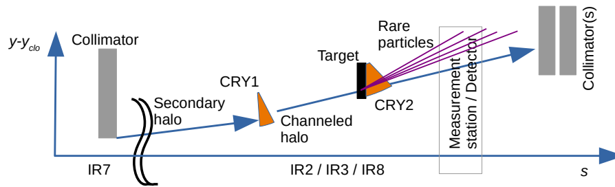
Figure 1: Double-crystal setup: the secondary beam halo scattered out of the primary collimator in the LHC betatron collimation region IR7 is guided by the splitting crystal CRY1 onto a target (T) with adjacent CRY2. Particle detection is provided by an existing detector (IR2/IR8) or dedicated measurement station (IR3) equipped with spectrometer (SPEC). Collimator(s) further downstream finally absorb the channelled halo. The vertical axis shows the vertical position w.r.t. the closed orbit y_{clo} .
