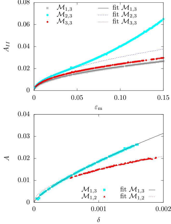
Figure 7: Values of A_{II} for \mathcal{M}_{\ell,m} as a function of \epsilon_m (top) and \delta (bottom) and their power-law fits, A_{II} \propto \epsilon_m^{1/2} \delta^{m/4} , to compare with the prediction in [29]. For \mathcal{M}_{2,3} , the improved fit from Eq. (23) is also shown (top).
