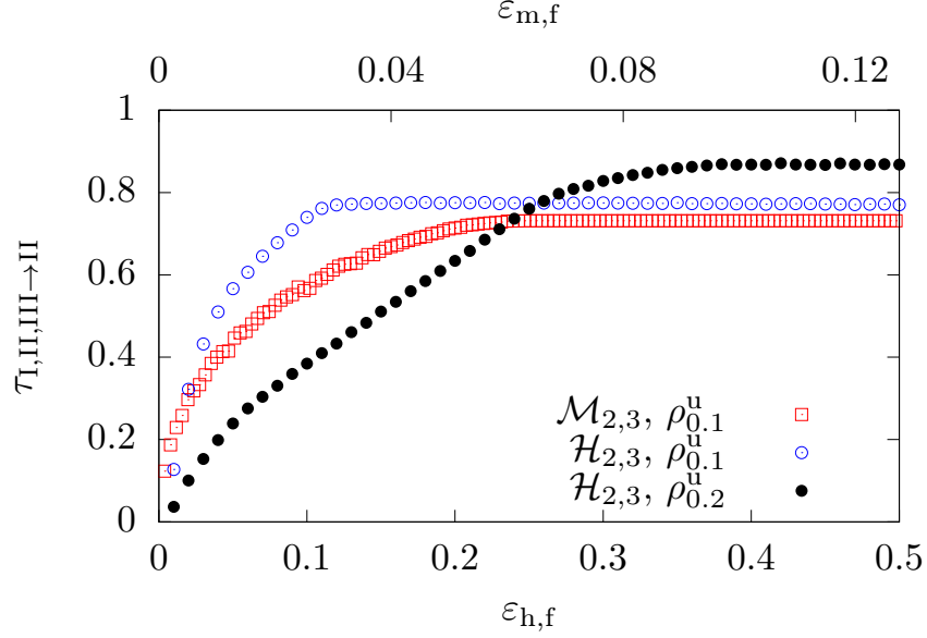
Figure 11: Trapping fraction for \mathcal{H}_{2,3} as a function of \epsilon_{h,f} (blue and black markers) and \mathcal{M}_{2,3} as a function of \epsilon_{m,f} (red), for initial uniform distributions with R = 0.1 and R = 0.2 . The two perturbation strengths are compared via the scaling \epsilon_{m,f} = \kappa^{3/2} \epsilon_{h,f} according to Eq. (14).
