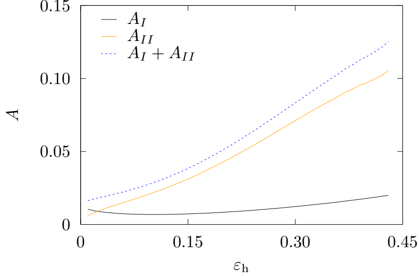
Figure 6: Areas of the center (black), islands (orange) areas, and their sum (blue, dotted) as a function of \varepsilon_h with k_3 = 1 , \omega_0/(2\pi) = 0.17133 , \omega = 2.995\omega_0 for \mathcal{H}_{2,3} .
