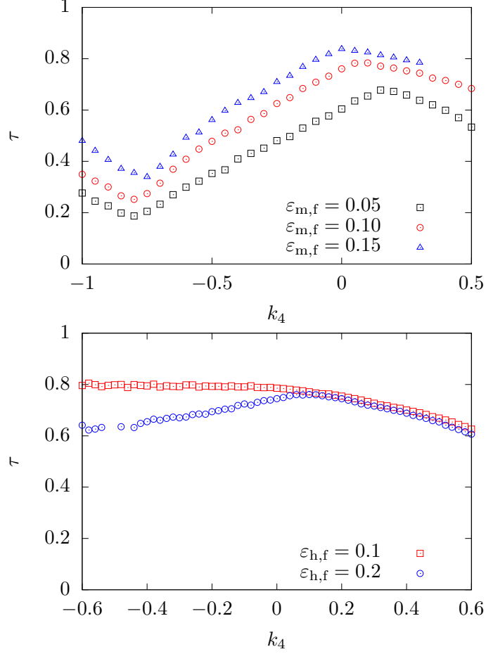
Figure 14: Top: trapping fraction for the model \mathcal{M}_{1,3} as a function of k_4 . Three cases with different values of \varepsilon_{m,f} are shown. Bottom: trapping for the model \mathcal{H}_{2,3} as a function of k_4 . Two cases with different values of \varepsilon_{h,f} are shown. In all cases, the initial distribution is uniform with R = 0.1 .
