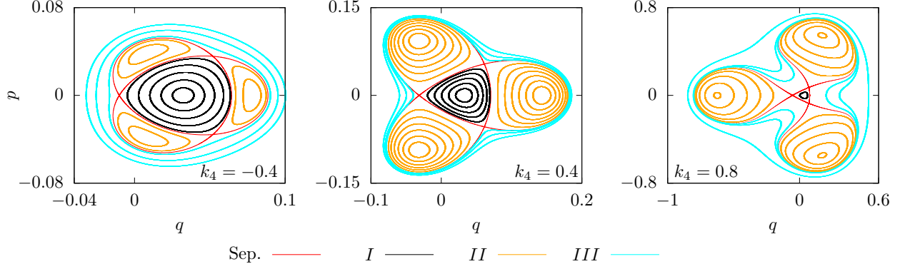
Figure 13: Phase-space portraits for \mathcal{H}_{1,3} in presence of different quartic nonlinearities k_4 , having set \omega_0/(2\pi) = 0.1713 , \omega = 2.995\omega_0 , \varepsilon = 0.28 . The portrait for k_4 = 0 is shown in Fig. 2 (bottom). Note the difference in scale of the three figures.
