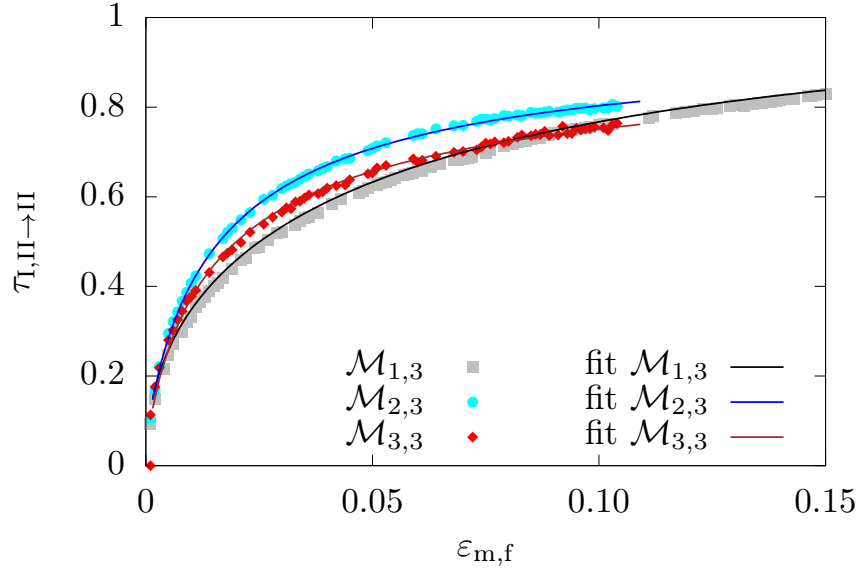
Figure 12: Trapping fraction for the models \mathcal{M}_{\ell,3} , \ell = 1, 2, 3 . Fits are presented based on Eq. (28), with A_I(\epsilon_m) = a + f(\epsilon_m, b, \epsilon_0) \epsilon_m^{-2/3} and A_{II}(\epsilon_m) = c \epsilon_m^{1/2} , in agreement with the models reported in Figs. 5 and 7.
