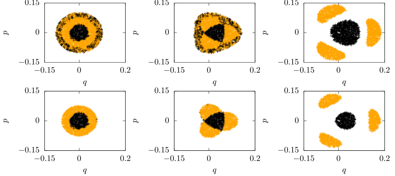
Figure 4: Evolution of an ensemble of particles in phase space with the colours used to identify in which region each initial condition has been trapped into (Region I, black, and Region II, orange) for the Hamiltonian model (4) with \ell = 1 , m = 3 at the beginning of the process (left column), at the end of the \varepsilon_h variation (mid column) and at the end of the frequency variation (right column). The difference between the top and bottom cases is the extent of the distribution of initial conditions: in the top case, some initial conditions are in Region III, while this is not the case for the bottom case. At large amplitudes, initial conditions can be either trapped in Region I or II in the top case, while this is absent in the bottom case. Parameters: k_3 = 1 , \omega_0/(2\pi) = 0.17133 , \omega_i = 2.995\omega_0 , \omega_f = 2.983\omega_0 , \varepsilon_{h,f} = 0.28 .
