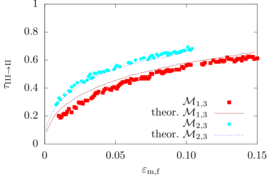
Figure 8: Comparison between the fraction of initial conditions in Region III and trapped in Region II as a function of \varepsilon_{m,f} , as computed with numerical simulations (markers) or using Eq. (1) (lines) for \mathcal{M}_{1,3} and \mathcal{M}_{2,3} . Note that the derivatives of the areas are estimated considering the finite difference for \omega_i = 2.995 \omega_0 and \omega_f = 2.983 \omega_0 having set k_3 = 1 , \omega_0/(2\pi) = 0.1713 .
