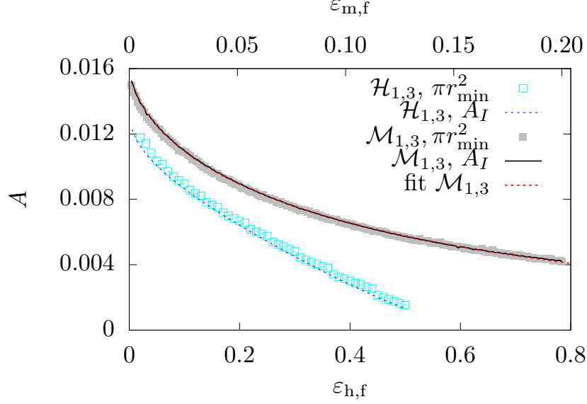
Figure 5: Comparison of the minimum enclosed area of trapped orbits and A_I at the end of the first stage, i.e. the linear variation of the exciter strength, as a function of \varepsilon_{h,f} , for \mathcal{H}_{1,3} with k_3 = 1 , \omega_0/(2\pi) = 0.17133 , \omega = 2.995\omega_0 , and for the corresponding map \mathcal{M}_{1,3} . A model of A_I(\varepsilon_m) = a + f(\varepsilon_m, b, \varepsilon_0)\varepsilon_m^{-2/3} fit for \mathcal{M}_{1,3} is presented, where f(\varepsilon_m, b, \varepsilon_0) is a form factor ( f(\varepsilon_m, b, \varepsilon_0) = b/[1 + (\varepsilon_0/\varepsilon_m)^{2/3}] ). The dynamics of \mathcal{H}_{1,3} has been simulated using N = 10^6 time steps.
