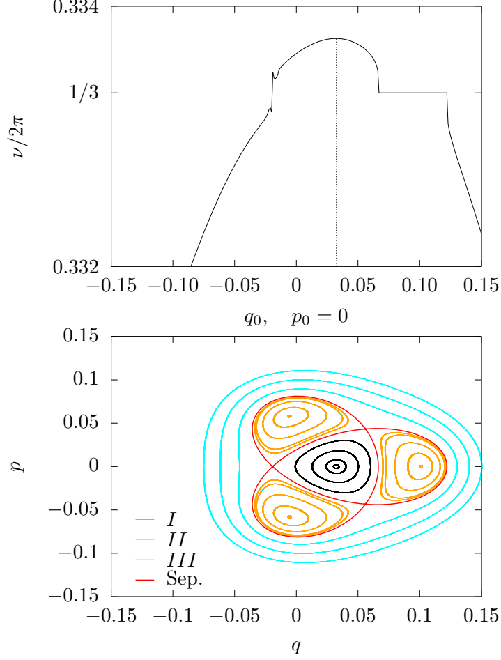
Figure 2: Top: Frequency \omega_0/(2\pi) evaluated with a high-accuracy FFT algorithm [36, 37] for an ensemble of orbits with initial conditions (q_0, 0) whose orbits are computed using the same model and parameters of the right plot. When the initial conditions are inside the resonance islands, the frequency is locked to the value 1/3 . Bottom: Phase-space portrait of the Poincaré map of the Hamiltonian \mathcal{H}_{1,3} (4) evaluated at \omega t = 2k\pi , k \in \mathbb{N} , for \omega_0/(2\pi) = 0.1713 , k_3 = 1 , \varepsilon_h = 0.28 , \omega = 2.995\omega_0 .
