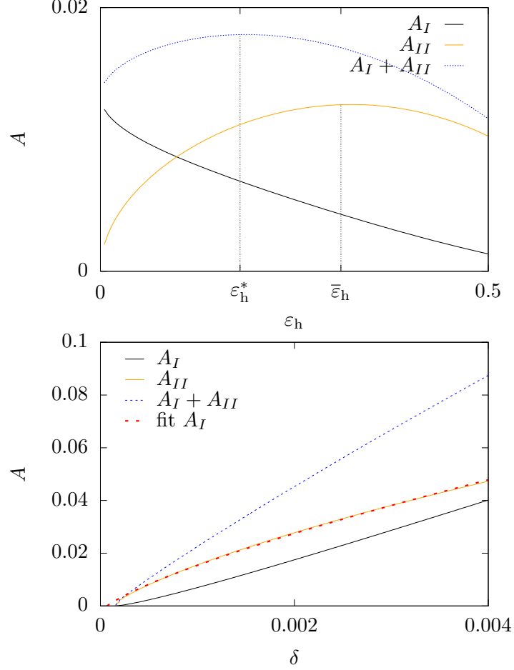
Figure 3: Top: Areas of Region I (black), Region II (orange) and of their sum (blue, dotted) as a function of the exciter strength \varepsilon_h , for k_3 = 1 , \omega_0/(2\pi) = 0.17133 , \omega = 2.995\omega_0 for \mathcal{H}_{1,3} . The sum of the areas has a maximum at \varepsilon_h^* whereas A_{II} has a maximum at a different point \bar{\varepsilon}_h . Bottom: Areas of Region I (black), Region II (orange) and of their sum (blue, dotted) as a function of the distance from the resonance \delta = 3\omega_0 - \omega with k_3 = 1 , \omega_0/(2\pi) = 0.17133 , \varepsilon_h = 0.28 for the Hamiltonian \mathcal{H}_{1,3} . A_{II} is fitted as \alpha\delta^{3/4} + \beta (red, dashed line) according to the predictions in [29].
