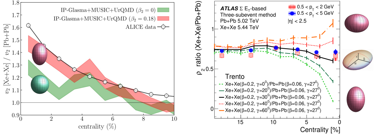
FIG. 3. Modification of multi-particle correlation observables in Xe+Xe collisions compared to the baseline with spherical nuclei provided by Pb+Pb collisions. Left: elliptic flow, v_2 [35]. Right: correlation between elliptic flow and the average transverse momentum, \rho_2 [45].
