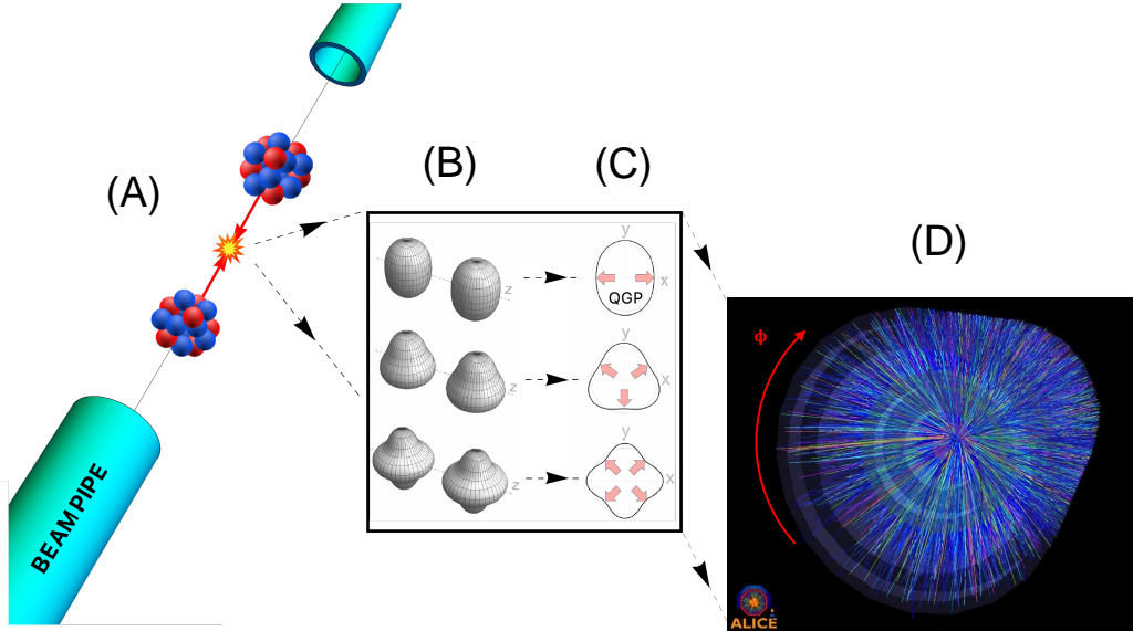
FIG. 1. Schematic view of a relativistic heavy-ion collision, highlighting the role played by the collective properties of the colliding ions in shaping the geometry of the produced quark-gluon plasma (QGP). The Lorentz contraction of the two nuclei in the z -direction, by factor \gamma \sim 100 at the BNL RHIC or over 1000 at the CERN LHC, is not shown. See text for a detailed description.
