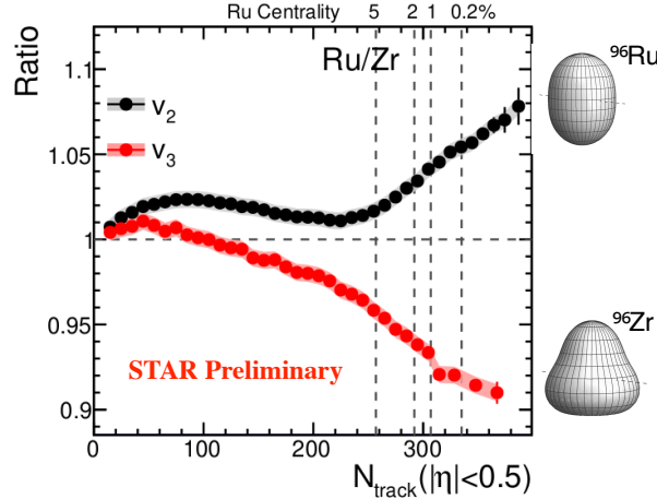
FIG. 4. Preliminary ratios of flow coefficients, v_n , taken between Ru+Ru and Zr+Zr collisions. The suppression of the v_3 ratio at large multiplicity is due to an enhancement of v_3 in Zr+Zr collisions.
