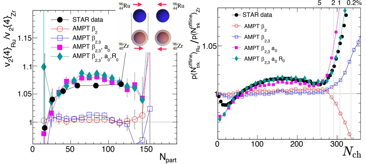
FIG. 5. Ratios of observables taken between Ru+Ru and Zr+Zr collisions. The inset in the left panel shows how the neutron excess of ^{96}\text{Zr} compared to ^{96}\text{Ru} yields a more diffuse nuclear surface, i.e., a larger a_0 and a slightly smaller R_0 in Eq. (1). Left: the impact of the larger a_0 of ^{96}\text{Zr} manifests predominantly in the fourth-order cumulant of v_2 , v_2\{4\} , which originates from the intrinsic ellipticity of the QGP due to the finite collision impact parameter. Right: both a_0 and R_0 differences contribute to a broad hump in the ratio of p(N_{\text{ch}}) . Calculations are obtained within the A Multi Phase Transport (AMPT) model [55].
