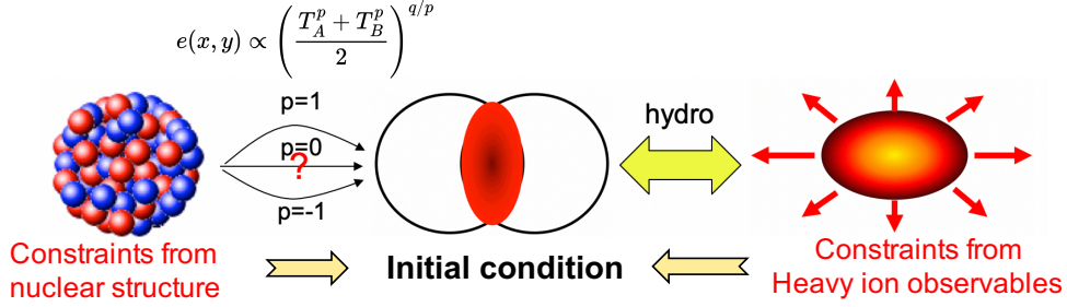
FIG. 6. Impact of isobar-like collisions on the goal of the heavy-ion program. Better control on the initial condition can be achieved by exploiting the constraints from both the ratios of final-state observables and the nuclear structure knowledge.
