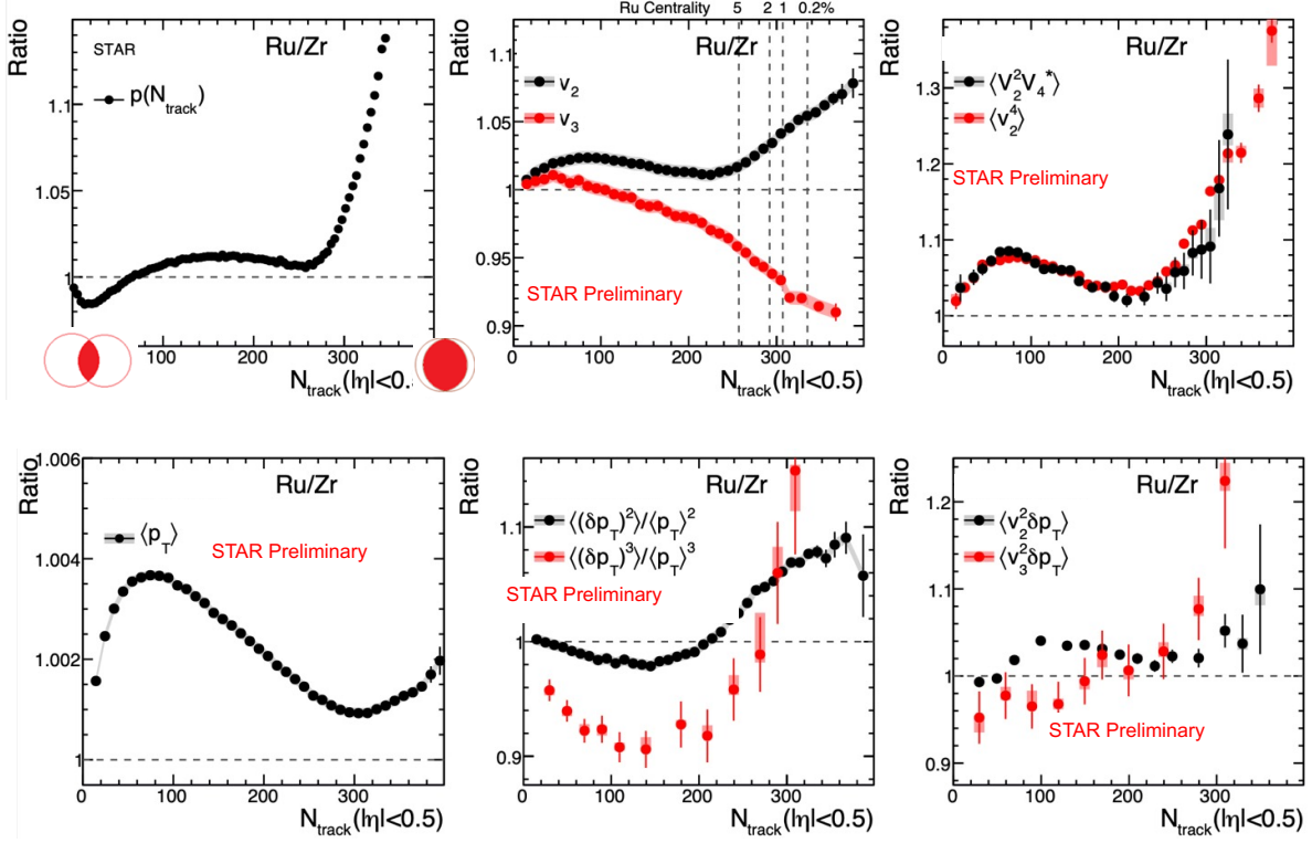
FIG. 2. Ratios of observables taken between ^{96}\text{Ru}+^{96}\text{Ru} and ^{96}\text{Zr}+^{96}\text{Zr} collisions as a function of N_{\text{ch}} , as measured by the STAR Collaboration (Preliminary results). A total of ten ratios are shown.
