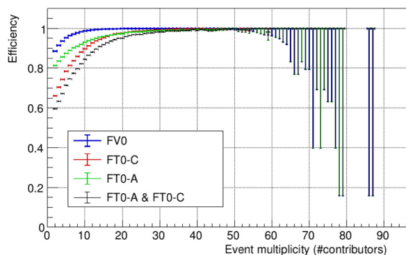
Fig. 8. The efficiency of a valid collision time reconstructed by different combinations of FIT detectors as a function of particle multiplicity.
