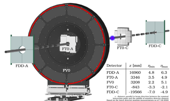
Fig. 1. Layout of FIT detectors. Inset shows the location along the beamline ( z ) and the pseudorapidity coverage ( \eta ) of each detector array.
