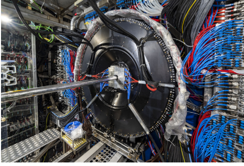
Fig. 3. Photograph of FVO and FT0-A after installation in ALICE.
