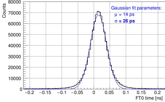
Fig. 4. FT0 collision time resolution.
