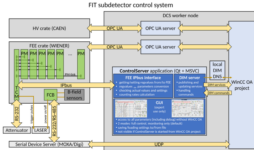
Fig. 2. Schema of the front-end electronics and its interfaces with the detector control system.
