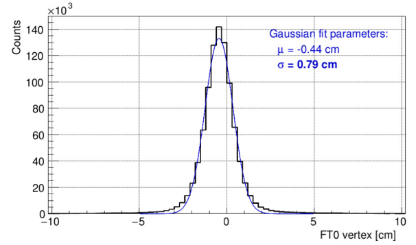
Fig. 6. FT0 vertex resolution.
