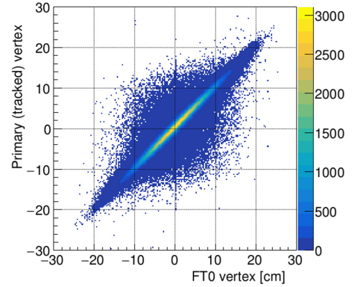
Fig. 7. Correlation between collision vertex reconstructed by the tracking detectors and FT0.
