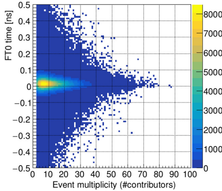
Fig. 5. Collision time distribution as a function of multiplicity.
