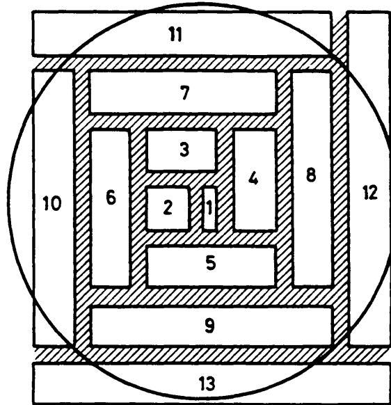
Fig. III.3 Filling of the horizontal phase plane by 13 slices when Q_H = 4.25 . Shaded area is the septum shadow.
