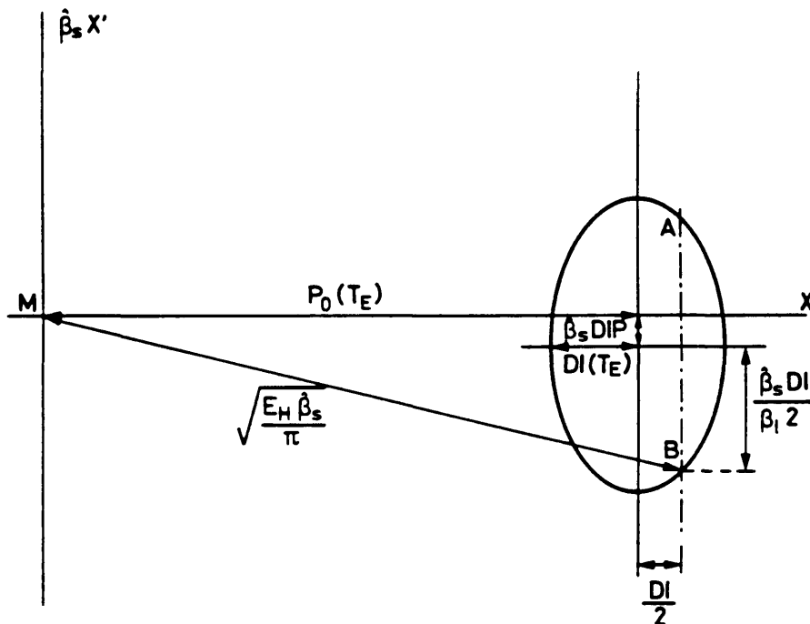
Fig. III.7 The position of the horizontal emittance limitation within the slice injected at time T_E .
