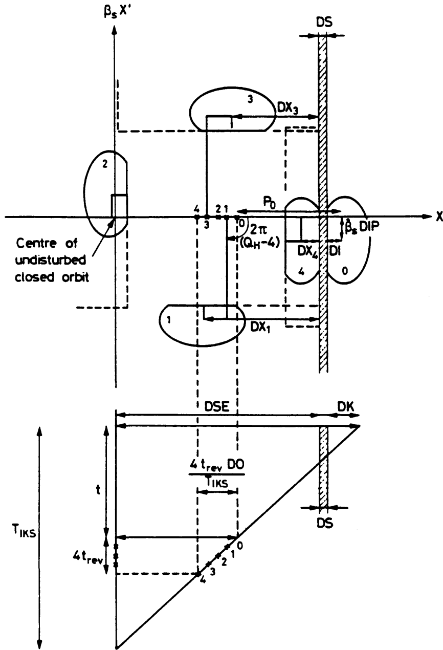
Fig. III.2 Evolution of a slice injected at point zero. Points 1, 2, 3, and 4 show the position of the slice after 1, 2, 3, or 4 turns, respectively, when Q_H = 4.25 (the value 4.25 is chosen to simplify the drawing).
