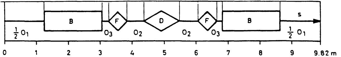
Fig. II.2 Phase advance \psi(s) and betatron functions \beta_H(s) and \beta_V(s) along one PSB period 3) .
