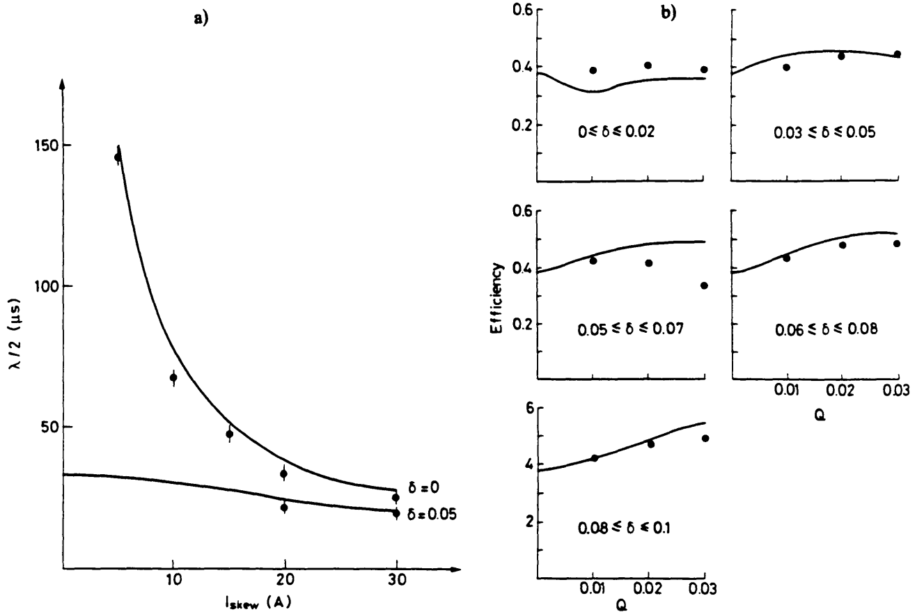
Fig. IV.5 a) Beating wavelength \lambda versus the skew quadrupole current I_{\text{skew}} , for two values of \delta , where \lambda = \sqrt{\delta^2/4 + Q^2} t_{\text{rev}} . Dots are measured values, solid lines are results of Eq. (IV.4). b) Multiturn injection efficiency versus Q . Dots represent measured values, solid lines are model predictions.
