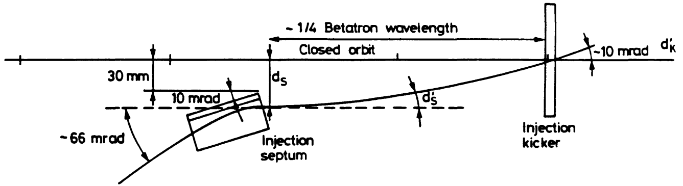
Fig. II.5 Monoturn injection into the PSB (schematic).
