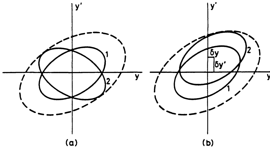
Fig. II.6 a) Emittance increase due to a mismatch of the incoming beam. b) Emittance increase due to a misalignment of the incoming beam.
