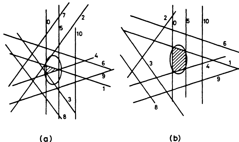
Fig. III.4 Layout of the septum cuts in the horizontal phase plane of two slices injected, with Q_H = 4.20 . The slice of (a) is injected at the start of the injection, while the slice of (b) is injected at the end.
