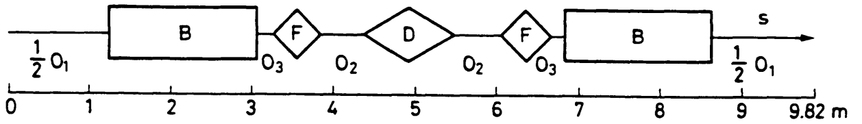
Fig. 1.4 Schematic diagram of one magnet period of a PSB ring 3) , B is a bending magnet; F and D are focusing and defocusing quadrupoles, respectively; O 1 , O 2 , and O 3 are field-free regions.
