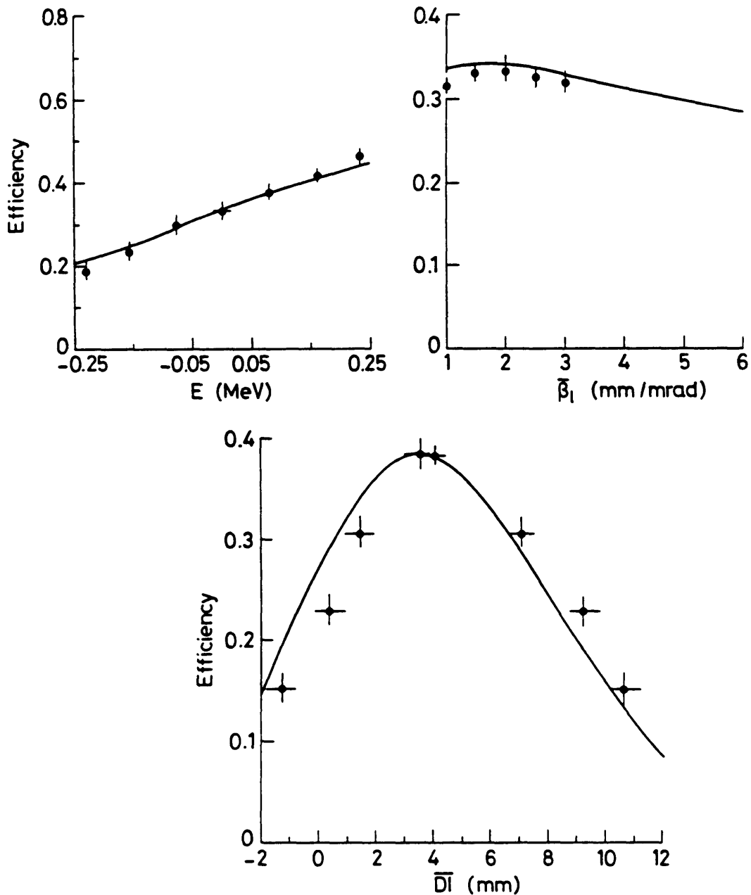
Fig. III.18 Plots of the efficiency versus the injection energy E , the injection focusing, and the injection alignment DI . Dots represent measured values, while the solid lines represent model predictions.
