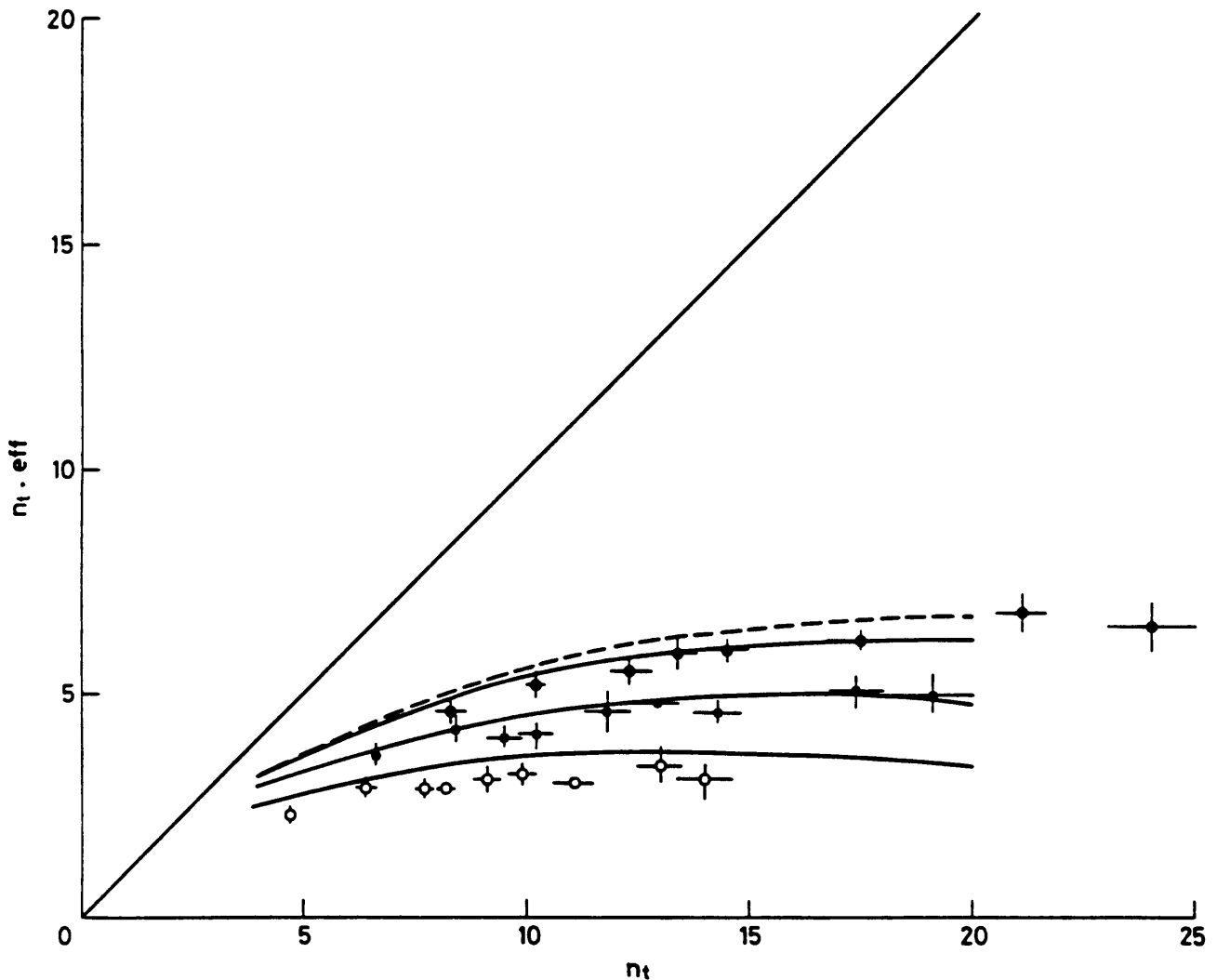
Fig. III.11 Plots of the measured number of effective turns ( n_t \cdot \text{eff} ) versus the number of injected turns ( n_t ) for E_H = 100, 130, and 160 \pi \text{ mm} \cdot \text{mrad} . The solid lines represent the calculated plots for the same three E_H values with DS = 3 \text{ mm} . The dotted line represents the same plot for E_H = 130 \pi \text{ mm} \cdot \text{mrad} when DS = 1.5 \text{ mm} .
