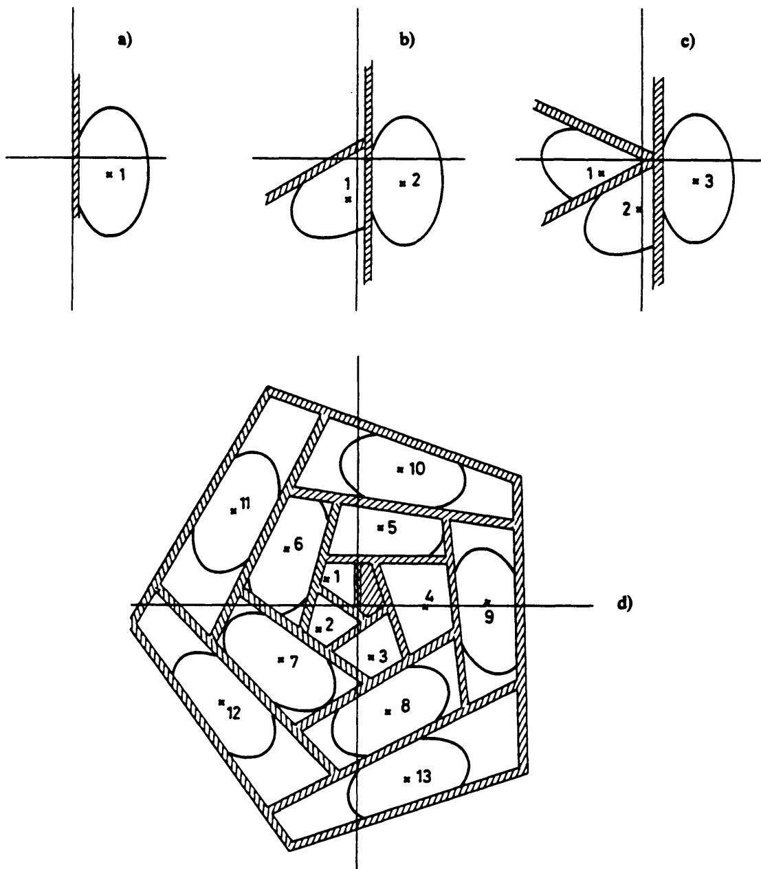
Fig. V.2 Evolution of the filling of the horizontal phase plane.
