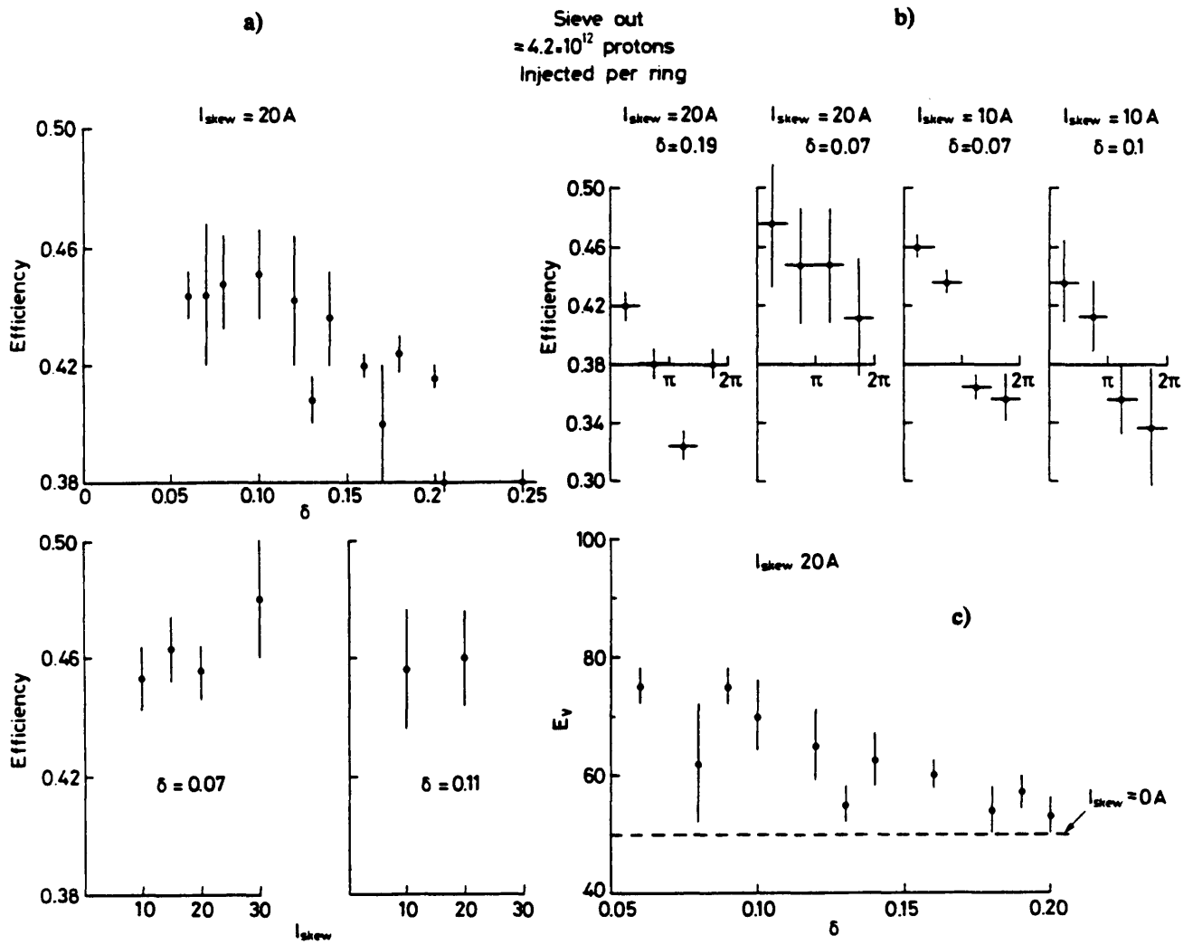
Fig. IV.6 a) Observed efficiency for high-intensity beam versus Q split \delta ; skew quadrupole current I_{skew} ( Eff = 0.38 for I_{skew} = 0 ). b) Efficiency versus the phase of the coupling term (for combinations of I_{skew} and \delta ). c) Vertical emittance E_v ( \pi \text{ mm} \cdot \text{rad} ) measured as a function of \delta .
