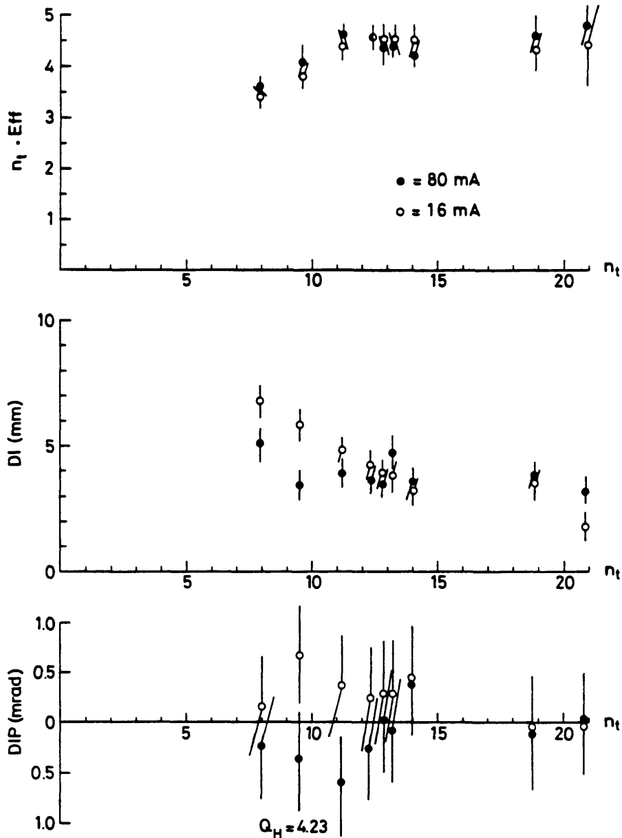
Fig. V.1 Plots of the measured number of effective turns ( n_t \cdot Eff ), and the beam alignment parameters ( DI and DIP ) versus the number of injected turns n_t . Open dots are low-intensity measurements. Closed dots are high-intensity measurements.
