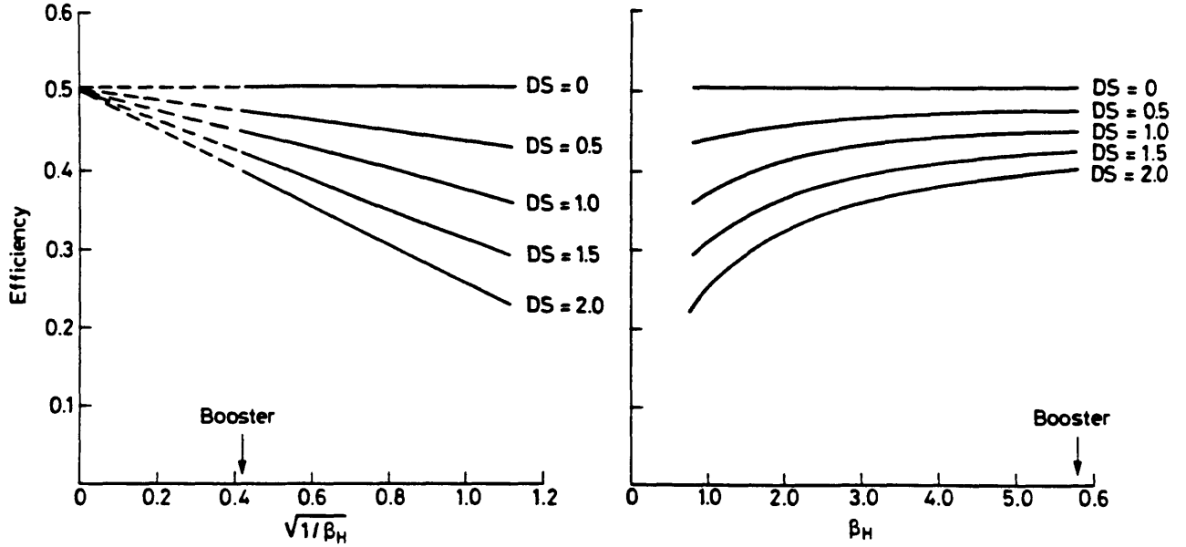
Fig. III.12 Plots of the calculated efficiency versus \beta_H and \sqrt{1/\beta_H} for five different DS values. The arrows indicate the \beta_H value of the PSB.
