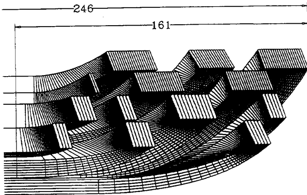
Fig. 2. Side view of end coils.
