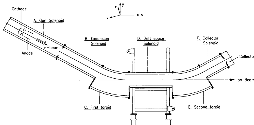
Figure 5: Electron Cooler General Layout
