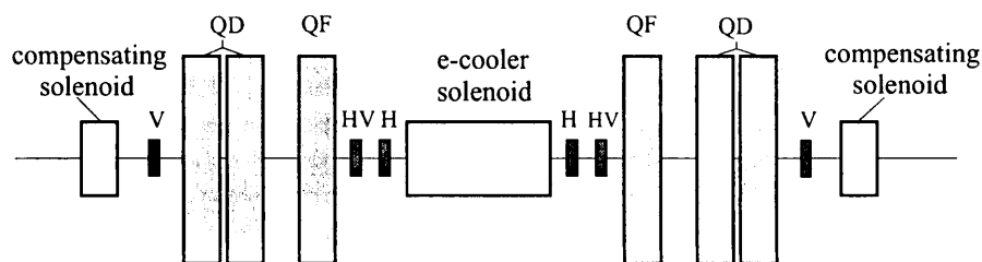
Figure 2. Schematic view of the AD electron cooling insertion
