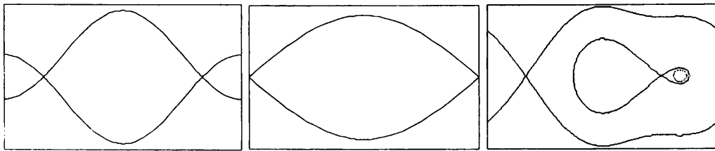
Figure 2: Bunch rotation stacking, longitudinal phase space plots (Energy versus Time): Left, Steady-state stacked bunch in decay mode. Middle, Injected and stacked bunches. Right, Start of bunch pair merging. The horizontal time axis on each plot is 25 ns.
