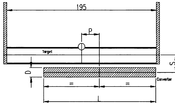
Fig. 1. A schematic view of target and converter assembly.
