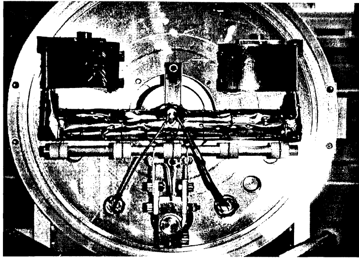
Fig. 6. Target UC 2 -C 183 before irradiation.
