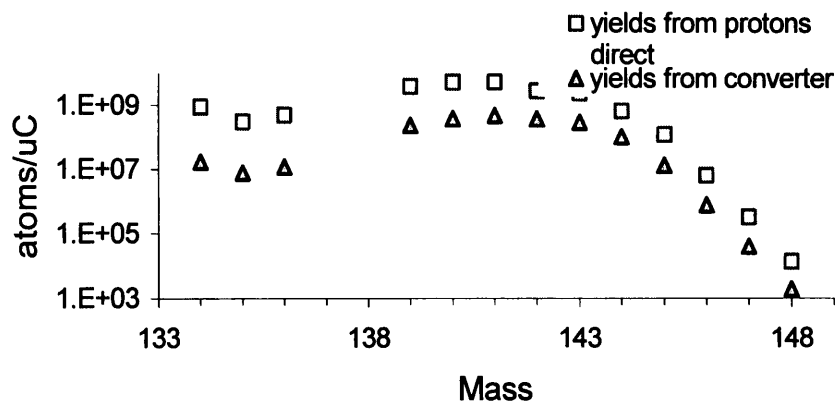
Fig. 2. Cs yields, from target UC 2 -C 183 , produced by protons directly on the target or from spallation neutrons.
